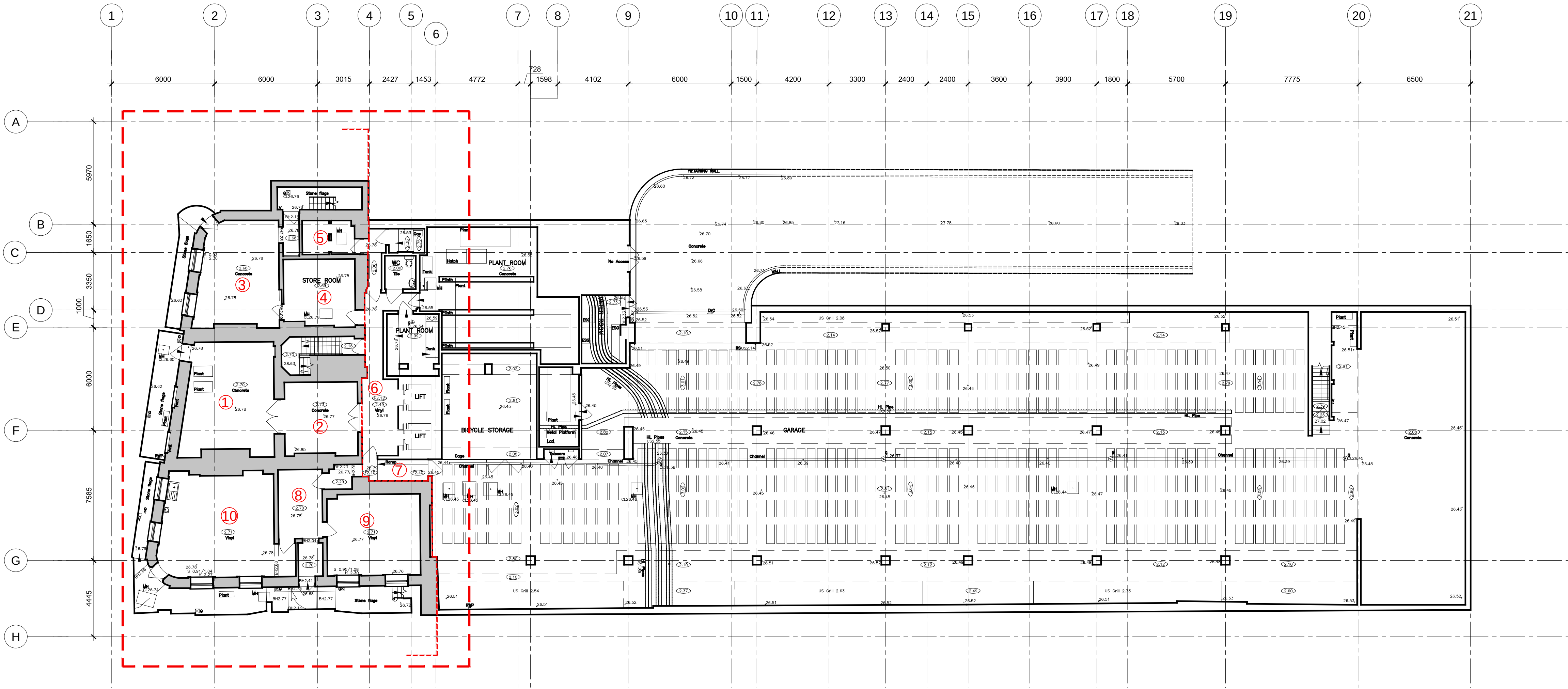
1 Basement Plan - Existing SCALE: 1:150 @ A0
