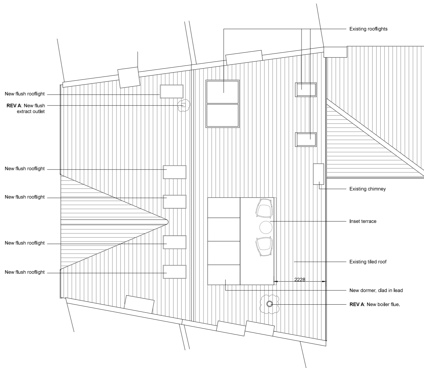
ROOF: PROPOSED
