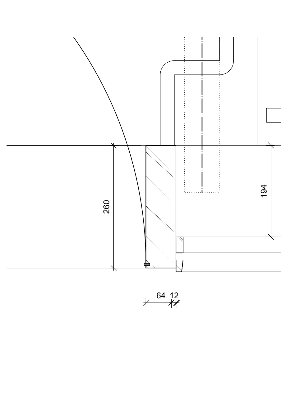
01 Society Offices Door and Cafe Door and Window Plan Details 1:5 - Read with 804
