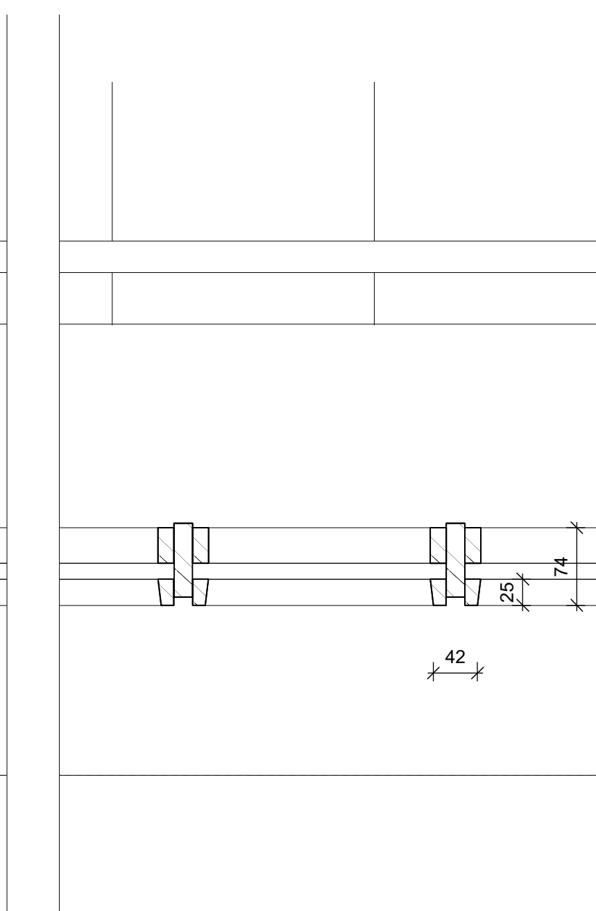
01 Society Offices Door and Cafe Door and Window Plan Details 1:5 - Read with 804
