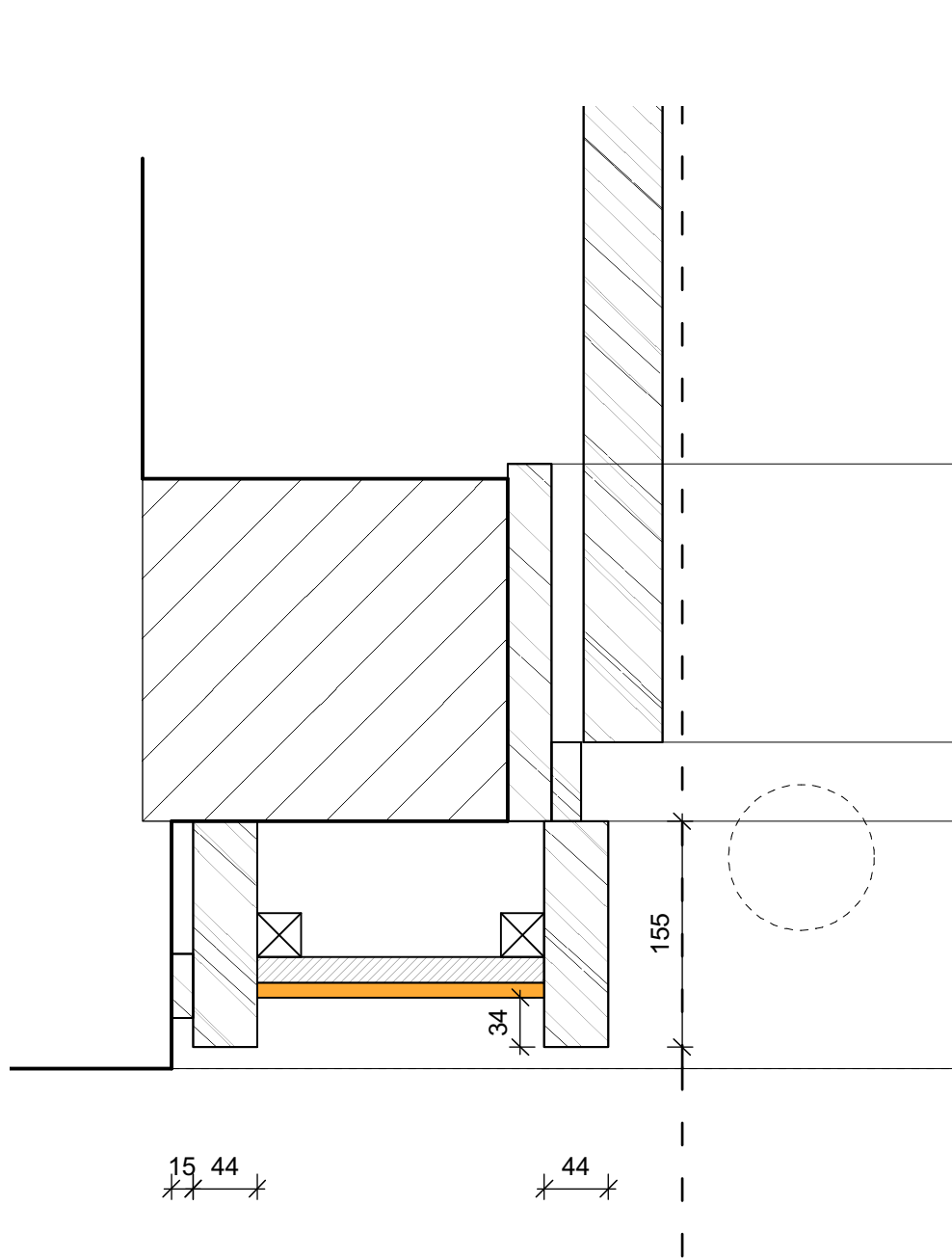
01 Society Offices Door and Cafe Door and Window Plan Details 1:5 - Read with 805
