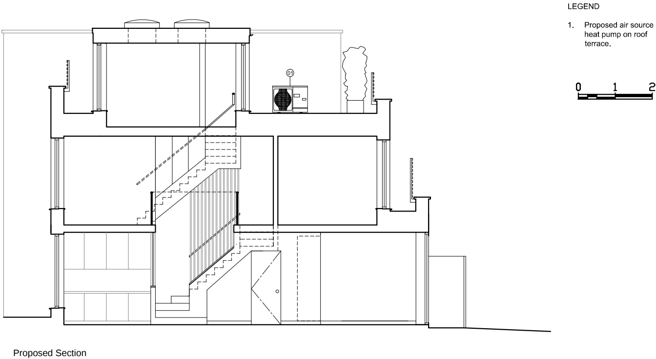
Proposed Section
