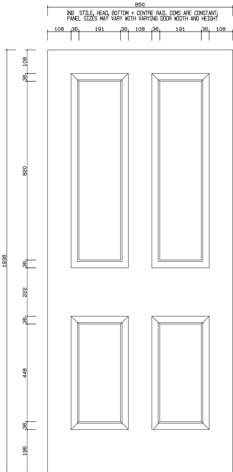
1:10 PAINTED SOFTWOOD DOOR (TYPICAL BUT HEIGHTS AND WIDTHS VARY) (FOR FULL SIZE DETAIL SECTIONS SEE DRAWING No 814.120)
