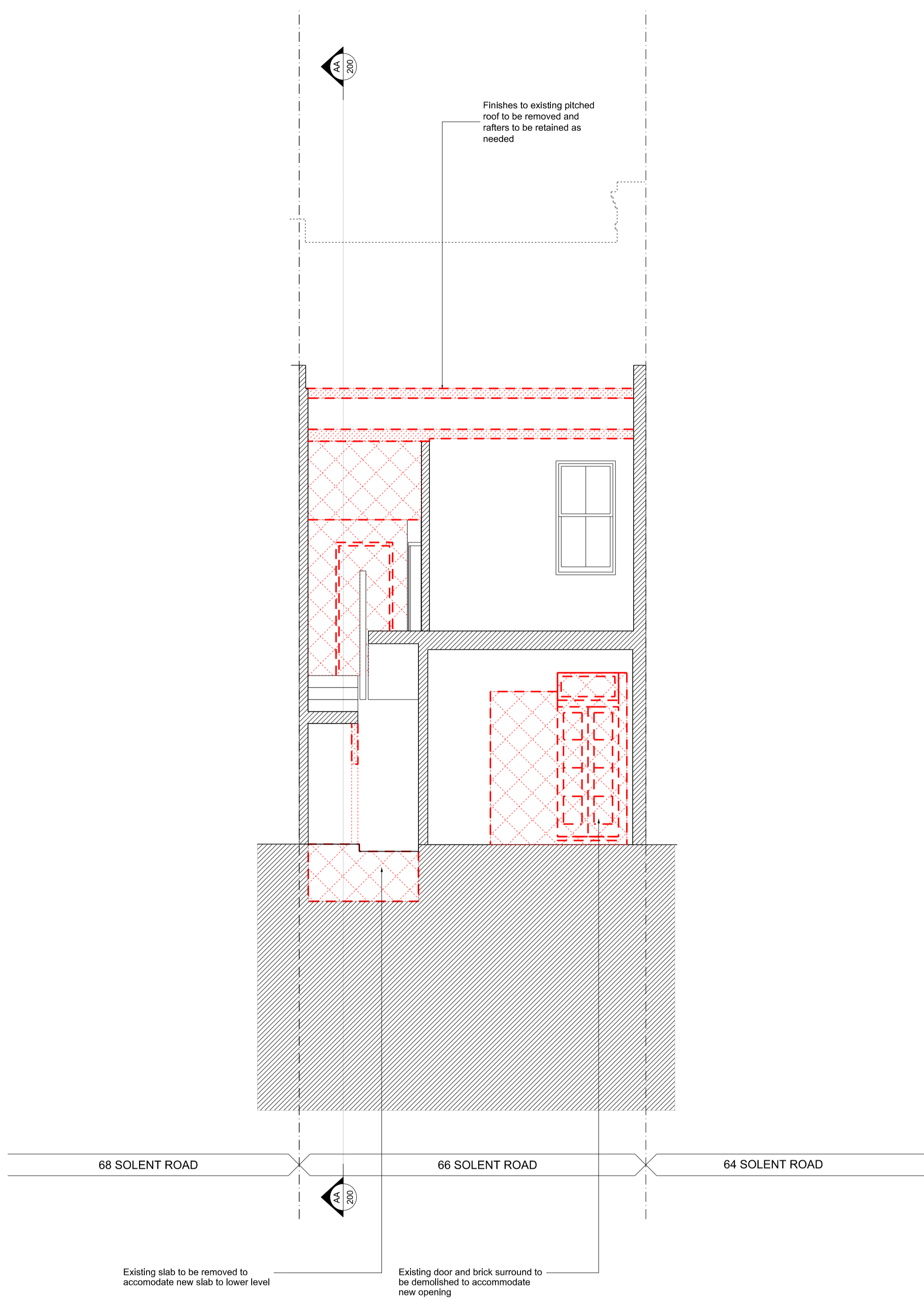
EXISTING & DEMOLITION SECTION B
