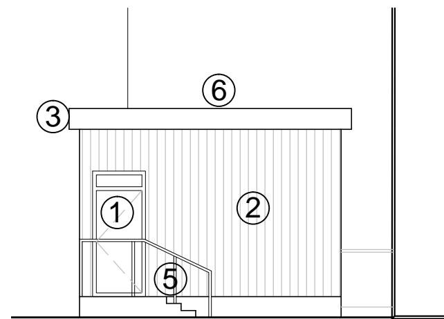
West Elevation
