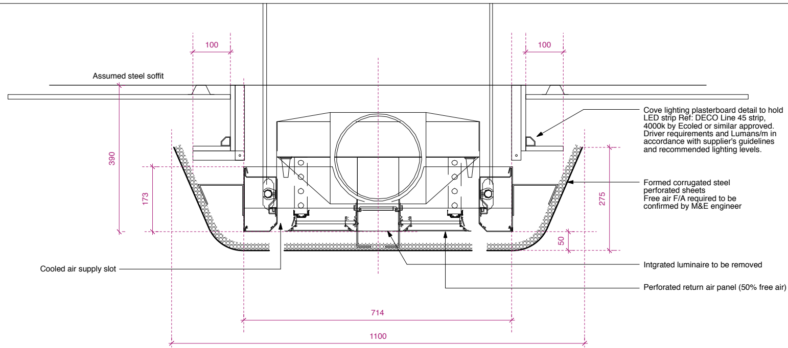
CHILLED BEAM COVER DETAIL (Scale 1:5)
