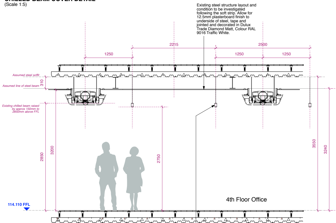
CHILLED BEAM AND SUSPENDED LIGHTING ARRANGEMENT
