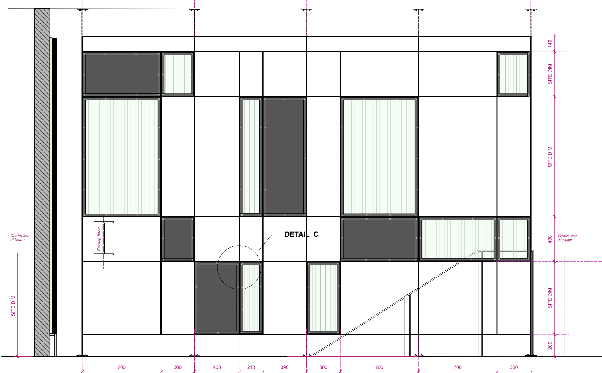
ELEVATION (Scale 1:10)
