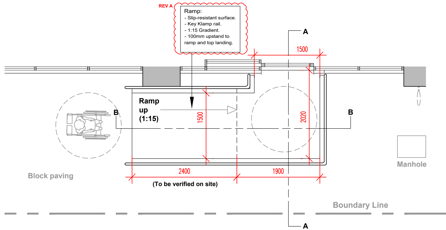
SITE PLAN (SCALE 1:50 @ A3)
