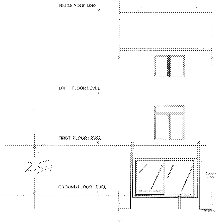
PROPOSED REAR ELEVATION PROPOSED REAR ELEVATION
