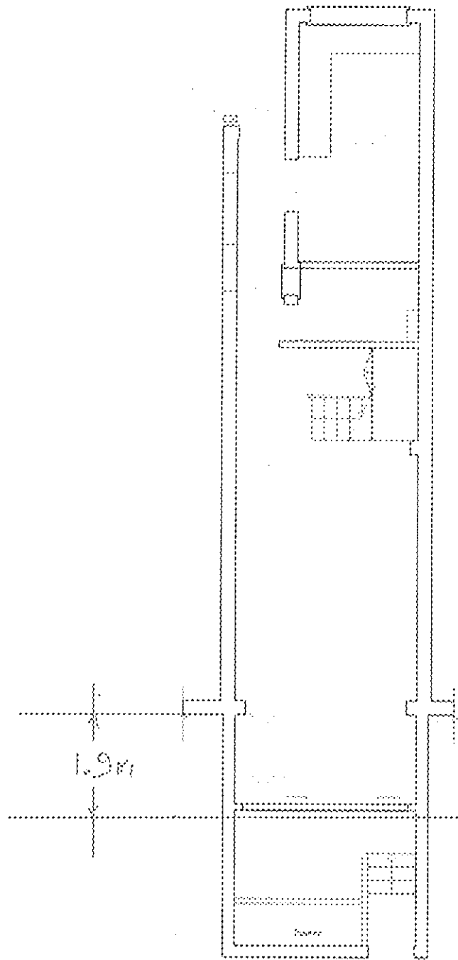
PROPOSED FLOOR PLAN NEW GROUND FLOOR PLAN
