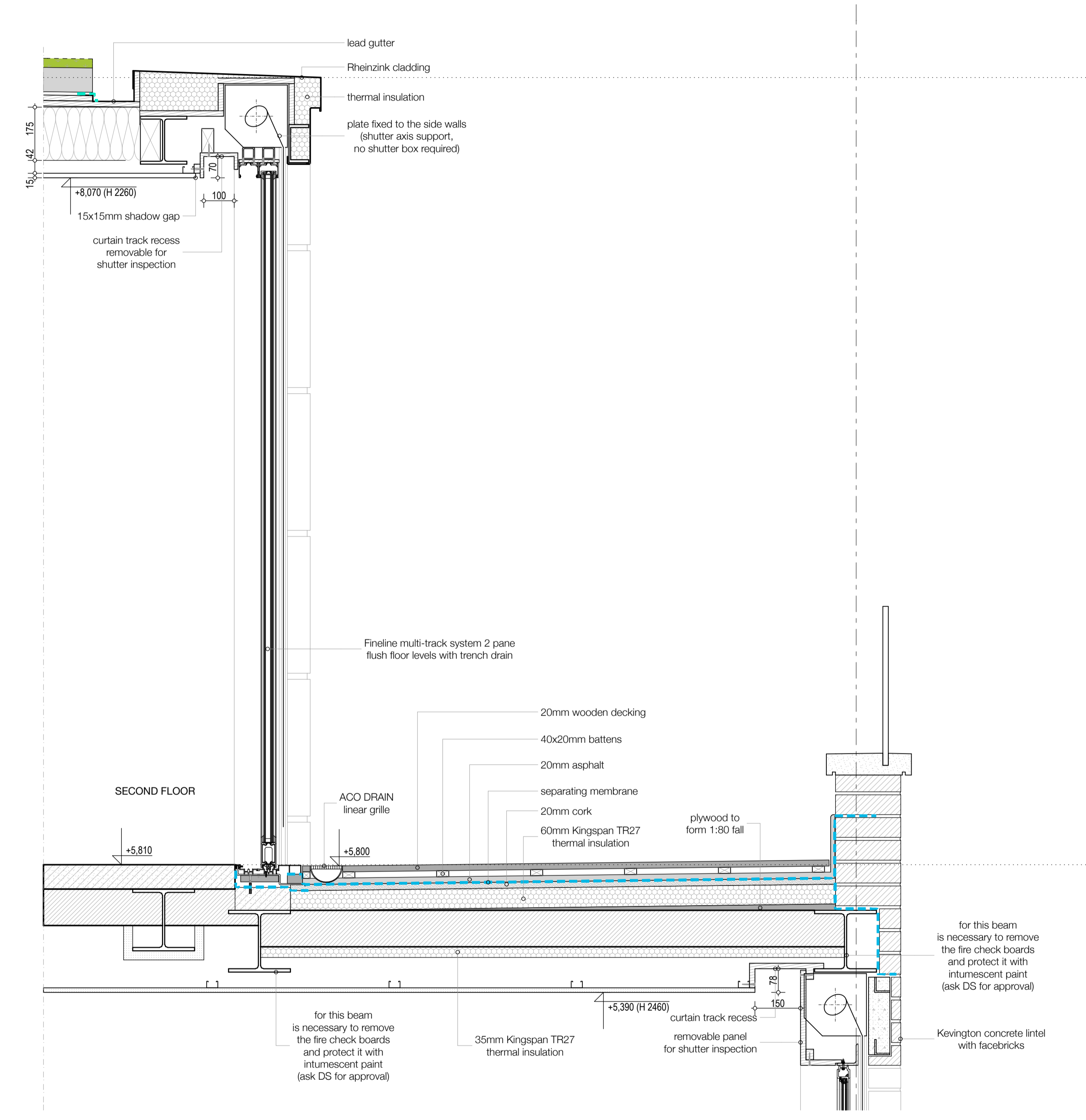
rear section external frames detail N 1:10
