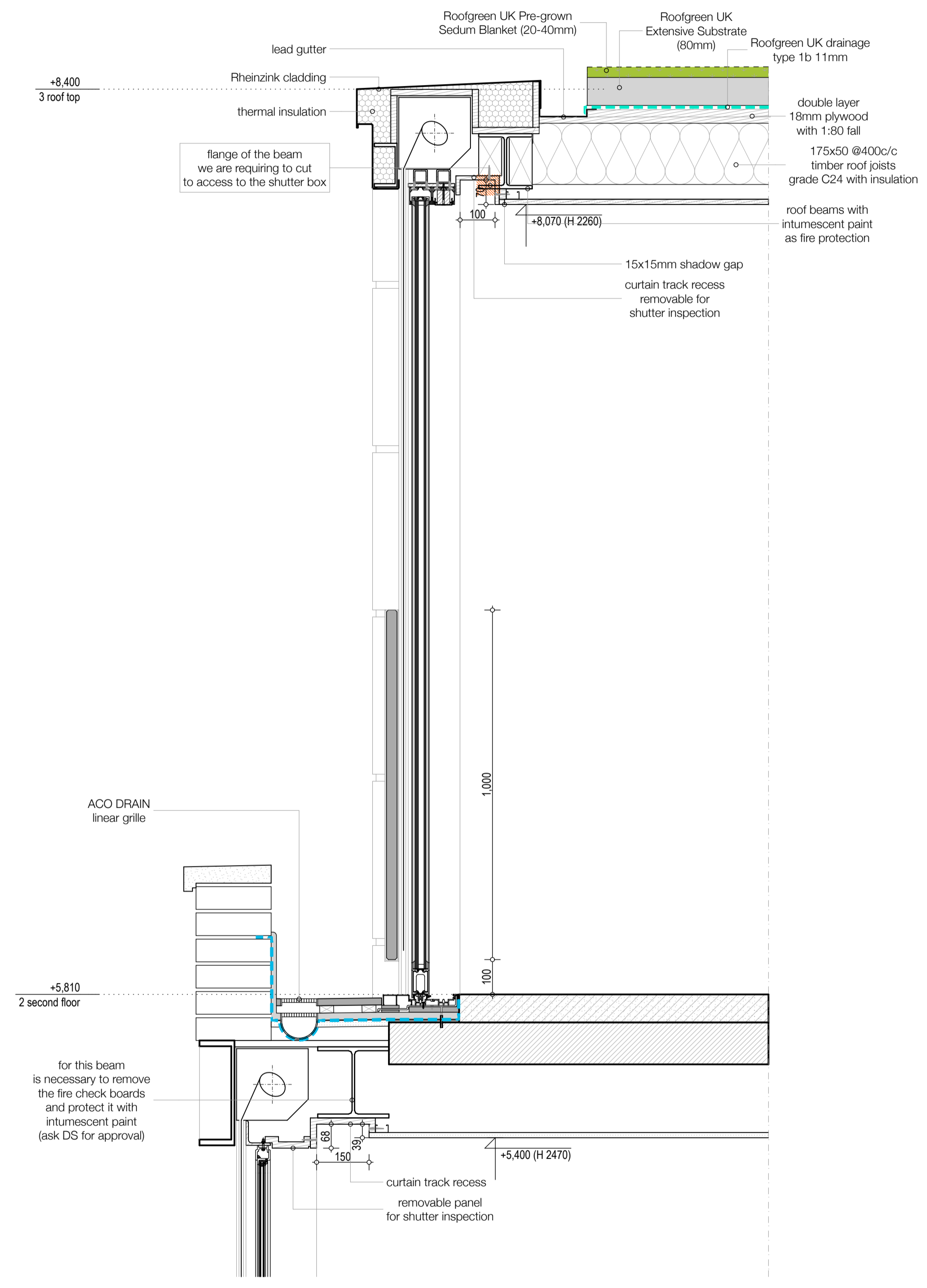
front section external frames detail M 1:10
