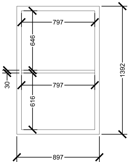
SECOND FLOOR WINDOW 22
