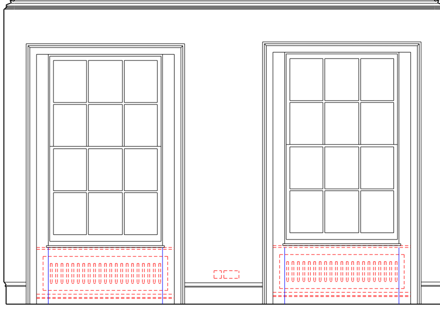
04 Master bedroom 18_02_01 Existing elevation west wall
