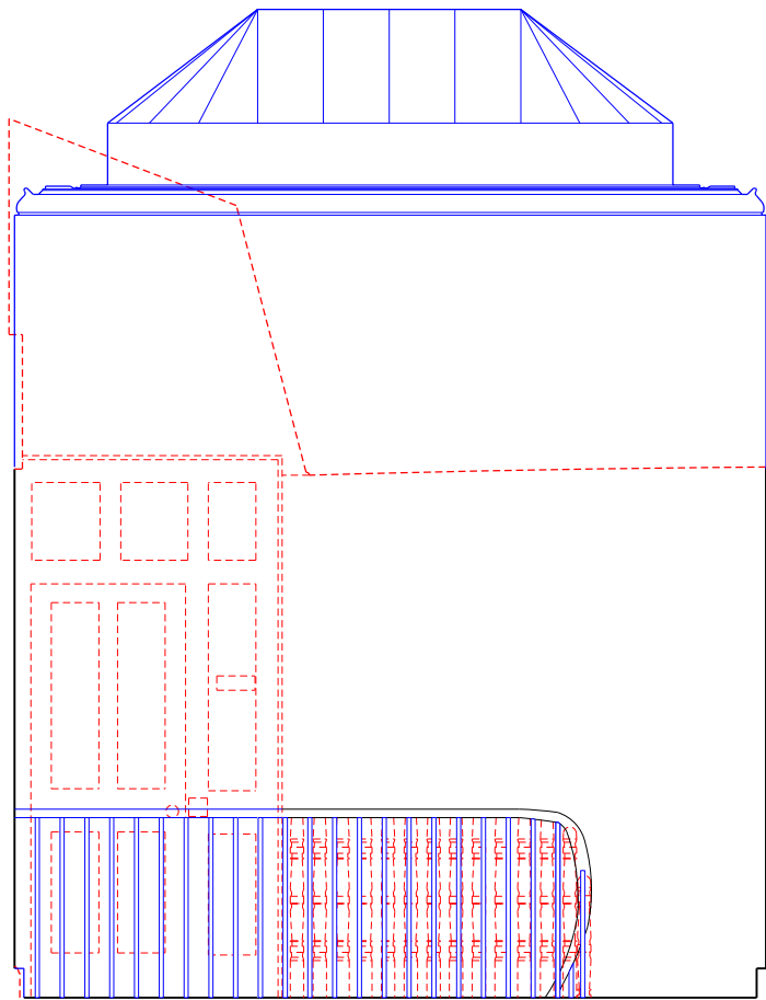
03 Stairwell 18_03_05 Elevation south wall
