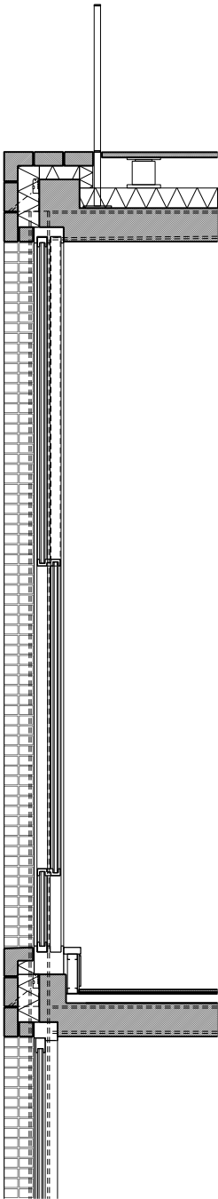
02 Section 21_01 Annex building
