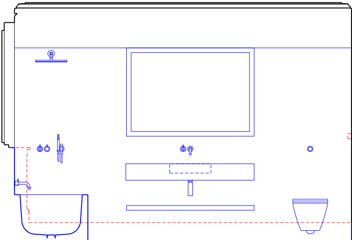
03 Bathroom 1 18_03_04 Elevation south wall
