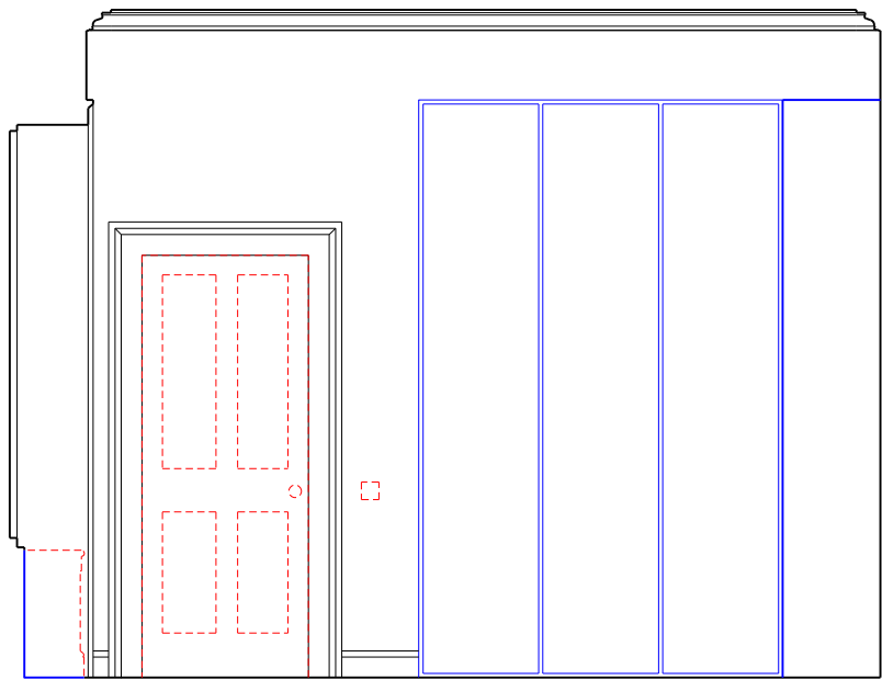
01 Master closet 18_02_03 Elevation north wall
