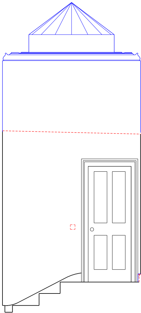
02 Stairwell 18_03_05 Elevation east wall
