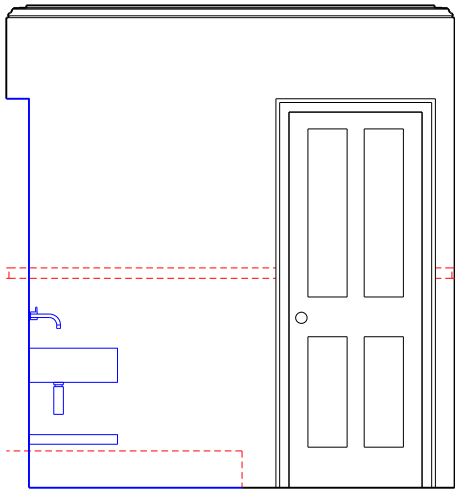
04 Bathroom 1 18_03_04 Elevation west wall
