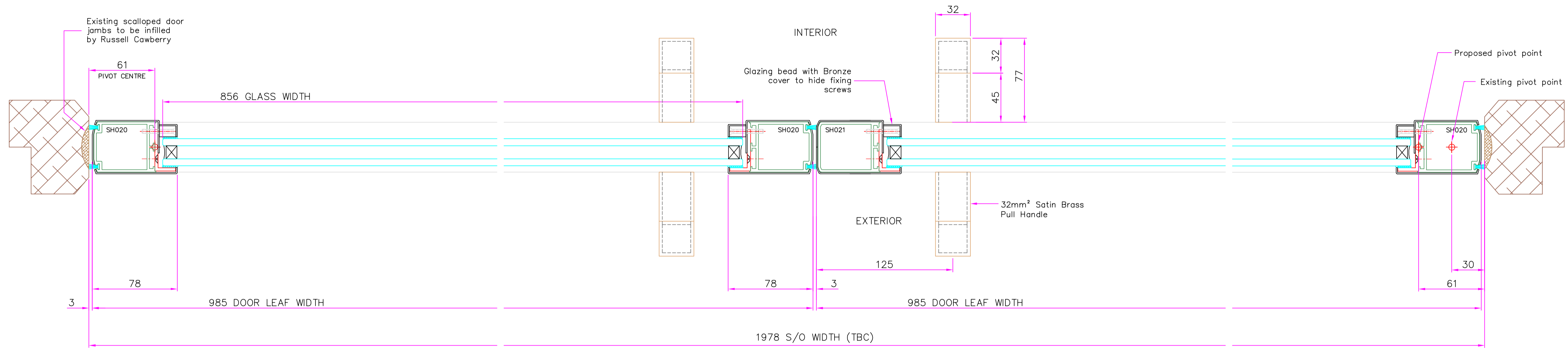
SECTION (S02.1)
