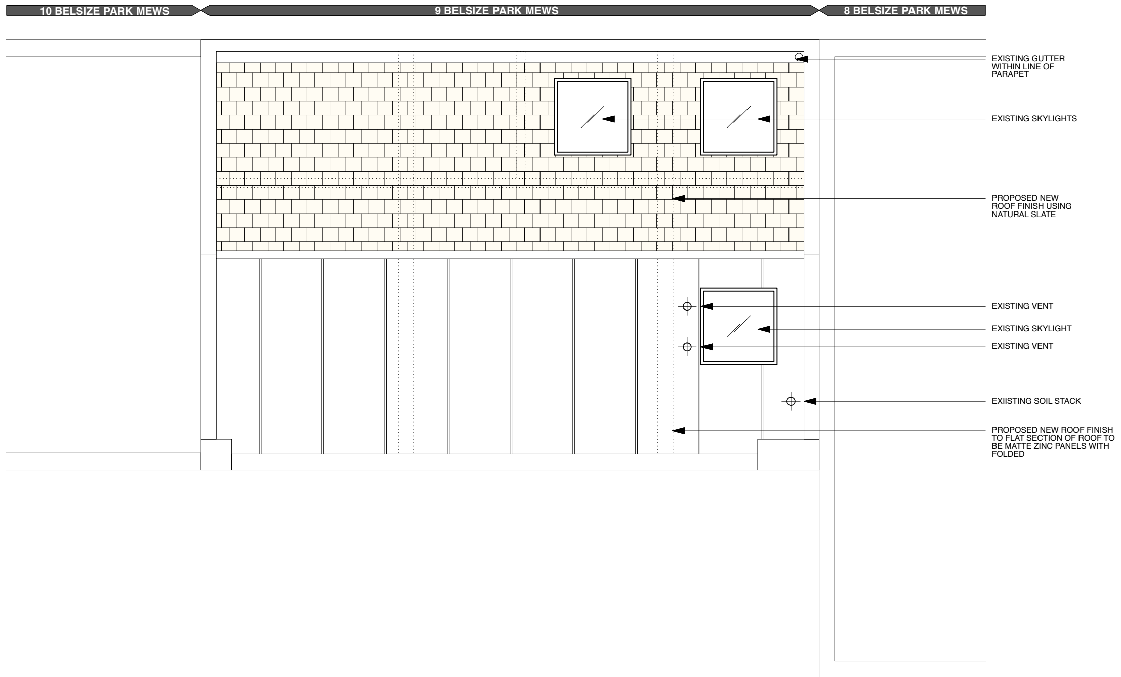
SCALE - 1:50
