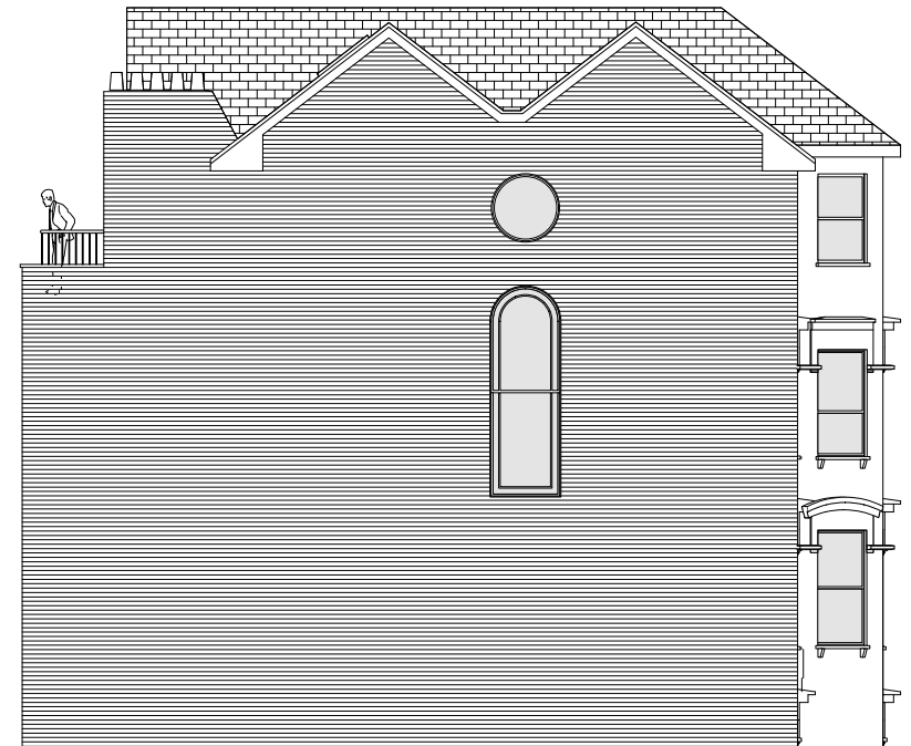
SIDE ELEVATION (SOUTH WEST)
