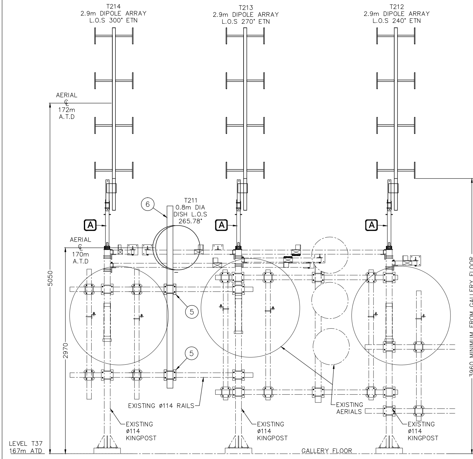
ENLARGED PART ELEVATION ON WEST FACE SCALE 1:20
