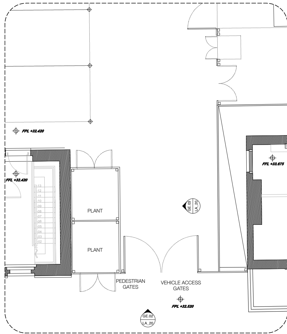
dE.02 Part Landscaping Plan CD.7.07 1:100@A3, 1:50@A1
