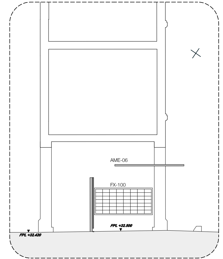
GS.01 Part Section (44 Gloucester Avenue) 1:100@A3, 1:50@A1
