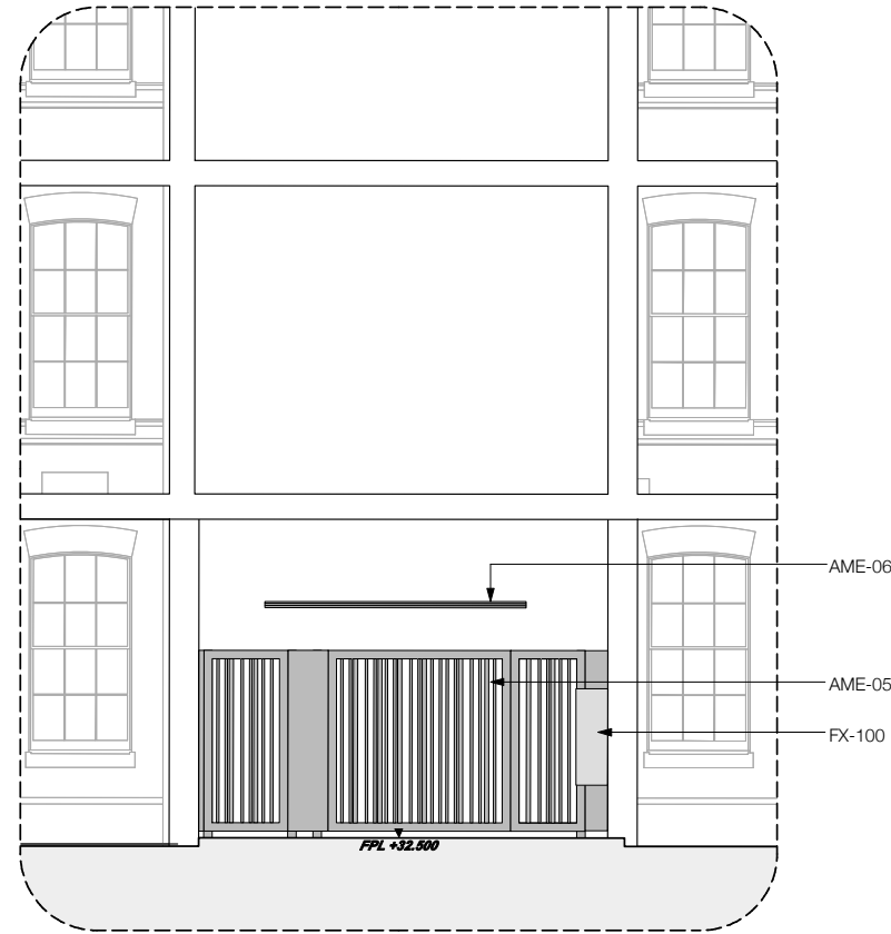
GE.01 Part Elevation 1:100@A3, 1:50@A1
