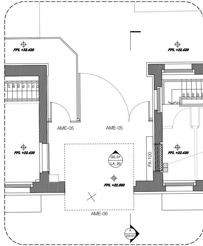
DE.01 Part Landscaping Plan 1:100@A3, 1:50@A1
