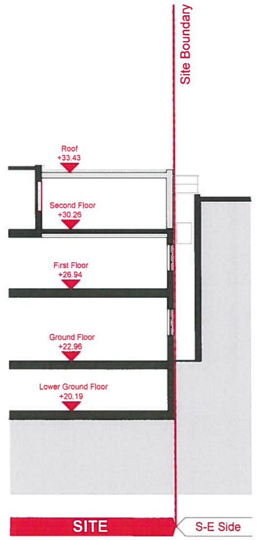
SECTION B-B
