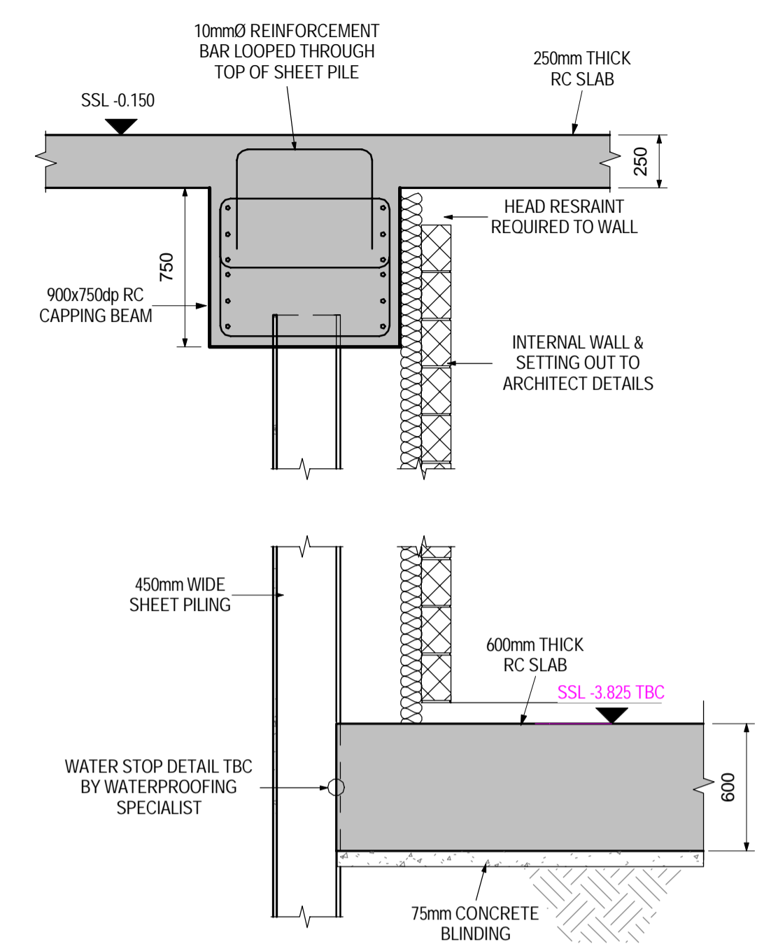
TYPICAL INTERNAL CAPPING BEAM DETAIL 04 SECTION 1 : 25
