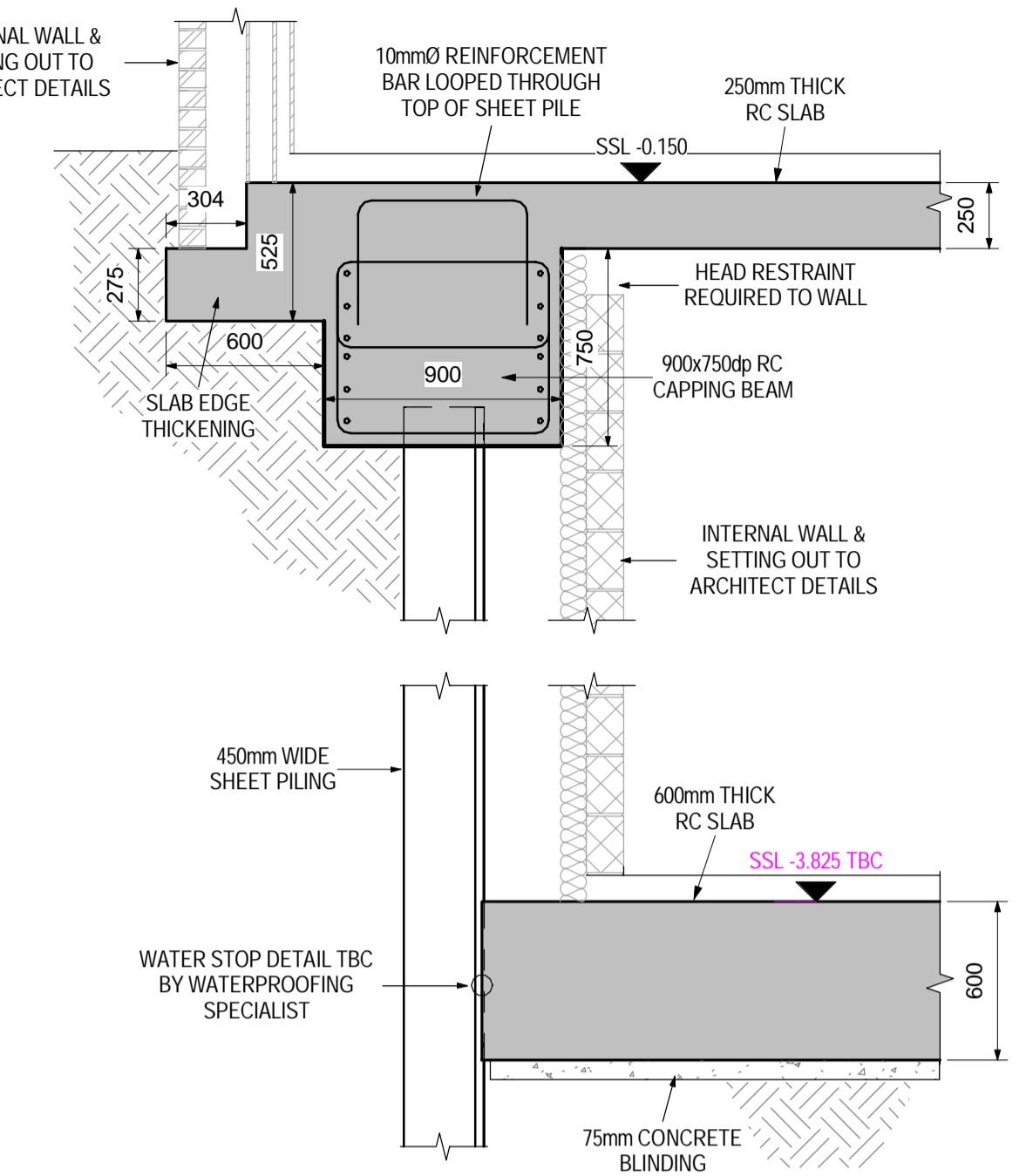
TYPICAL EXTERNAL CAPPING BEAM DETAIL 05 SECTION 1 : 25
