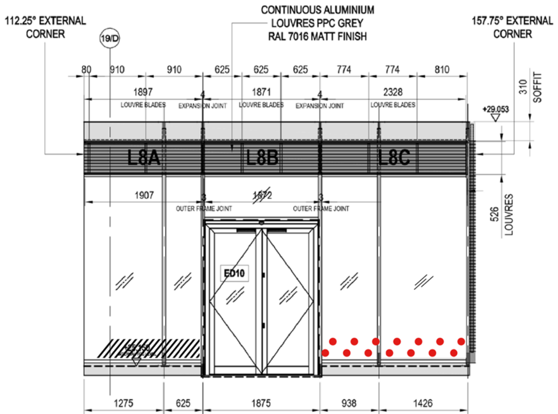
(L8) GROUND FLOOR LOUVRES - CORE 4
