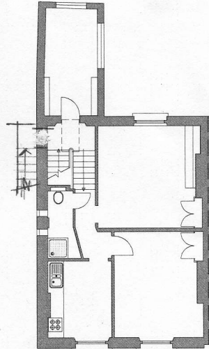
Proposed Layout - Second Floor
