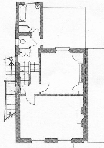
Proposed Layout - First Floor
