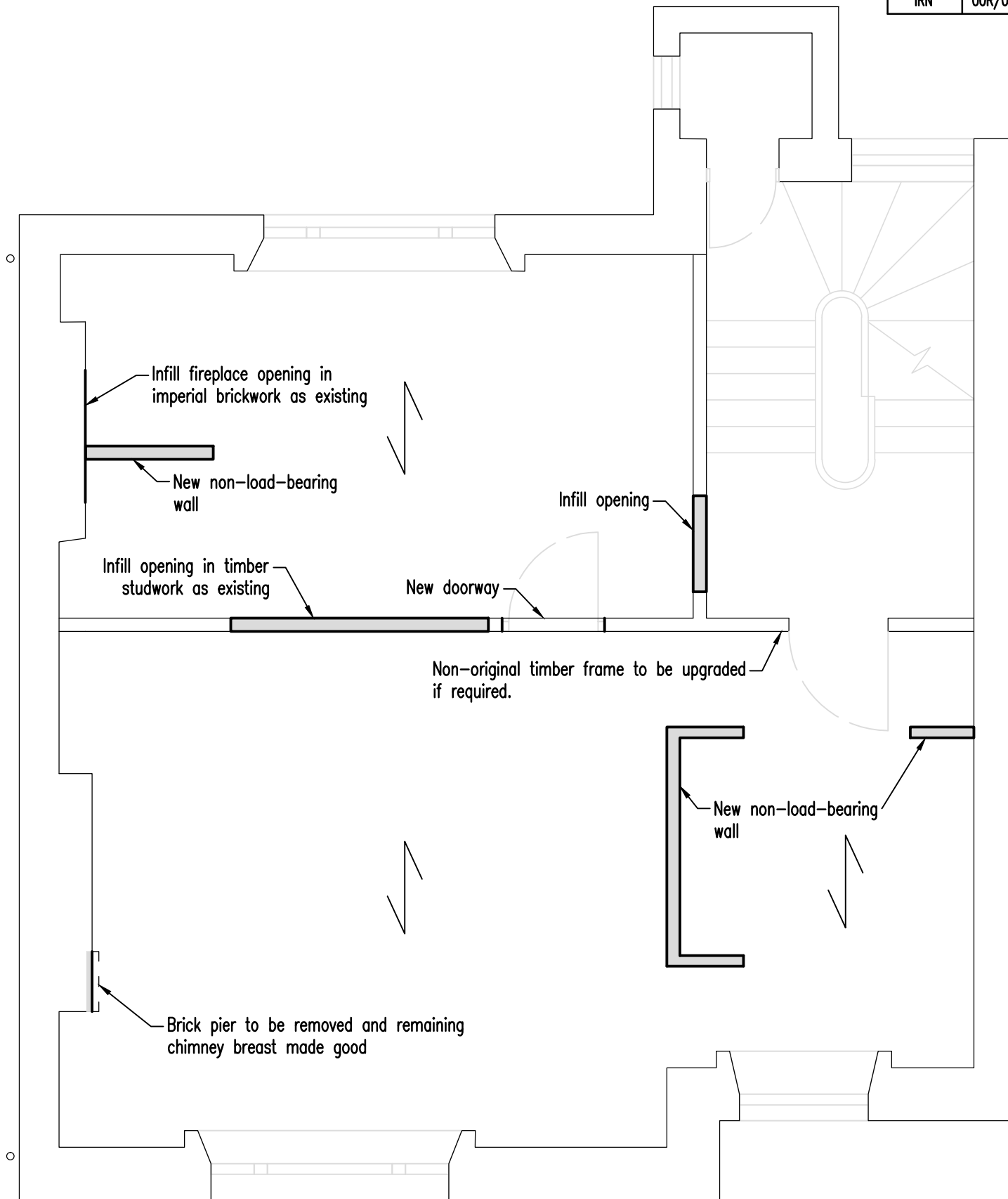
FIRST FLOOR REMEDIAL WORKS SCALE 1:50@A3
