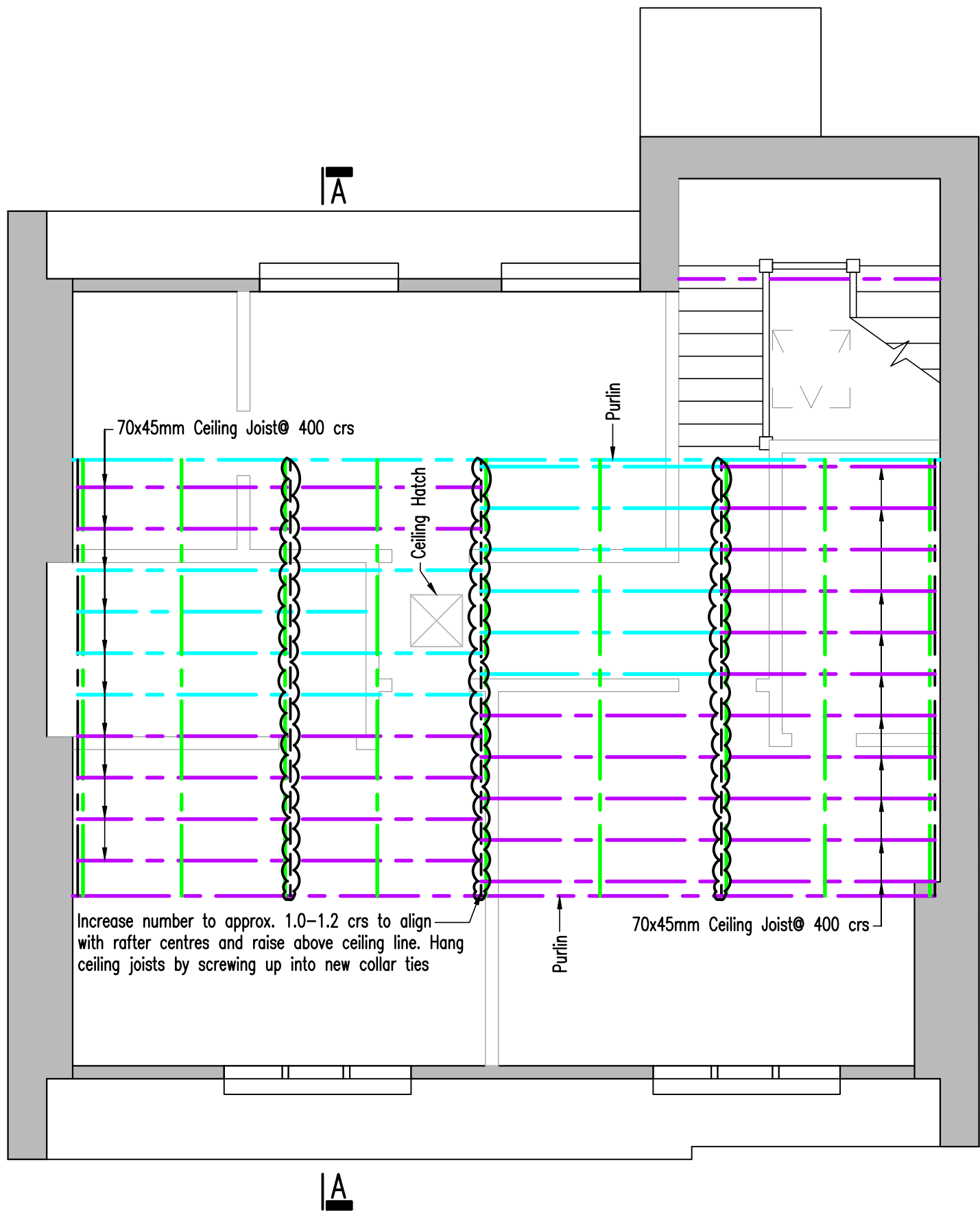
PROPOSED THIRD FLOOR PLAN, CEILING LEVEL SCALE 1:50@A3
