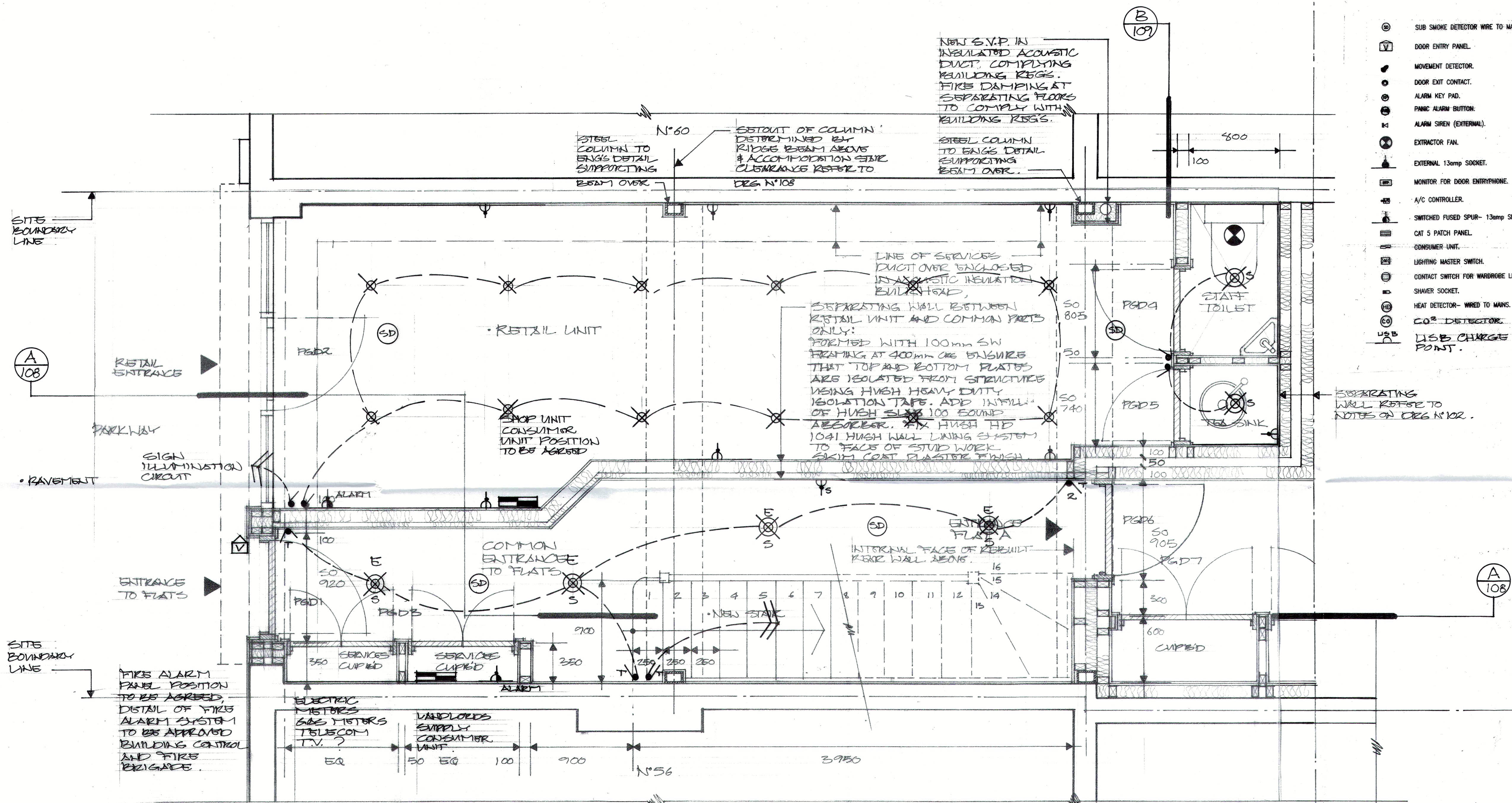
DETAIL PLAN FRONT SECTION OF GROUND FLOOR
