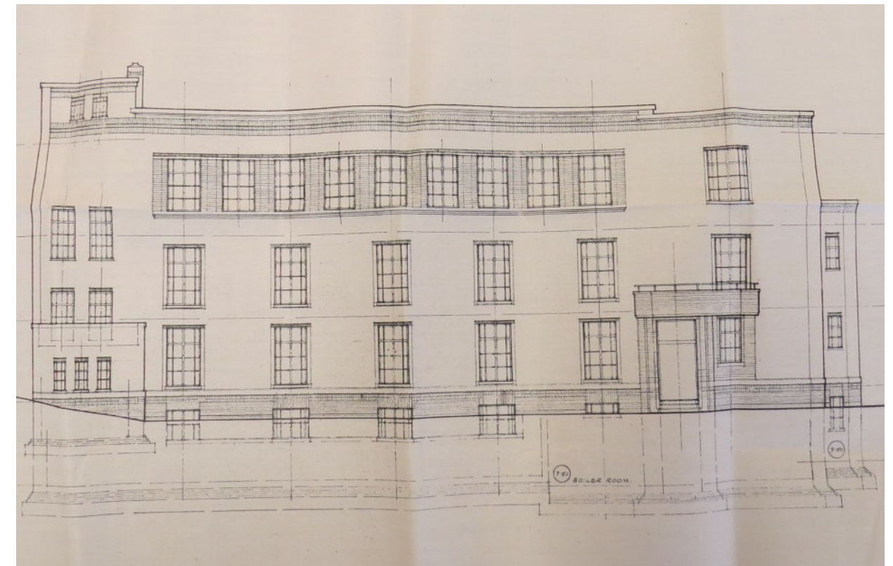
Figure 42 The west elevation produced for the new Lord Cameron Hall in 1934.
