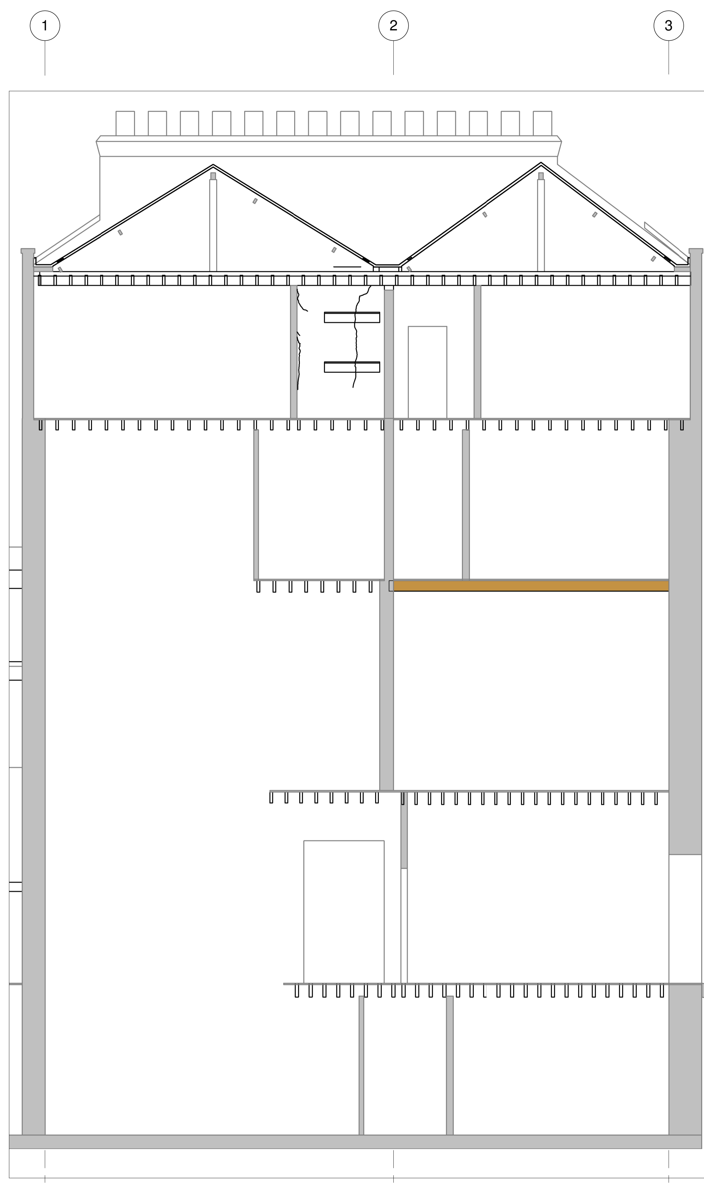
2 North Party Wall 1 : 50
