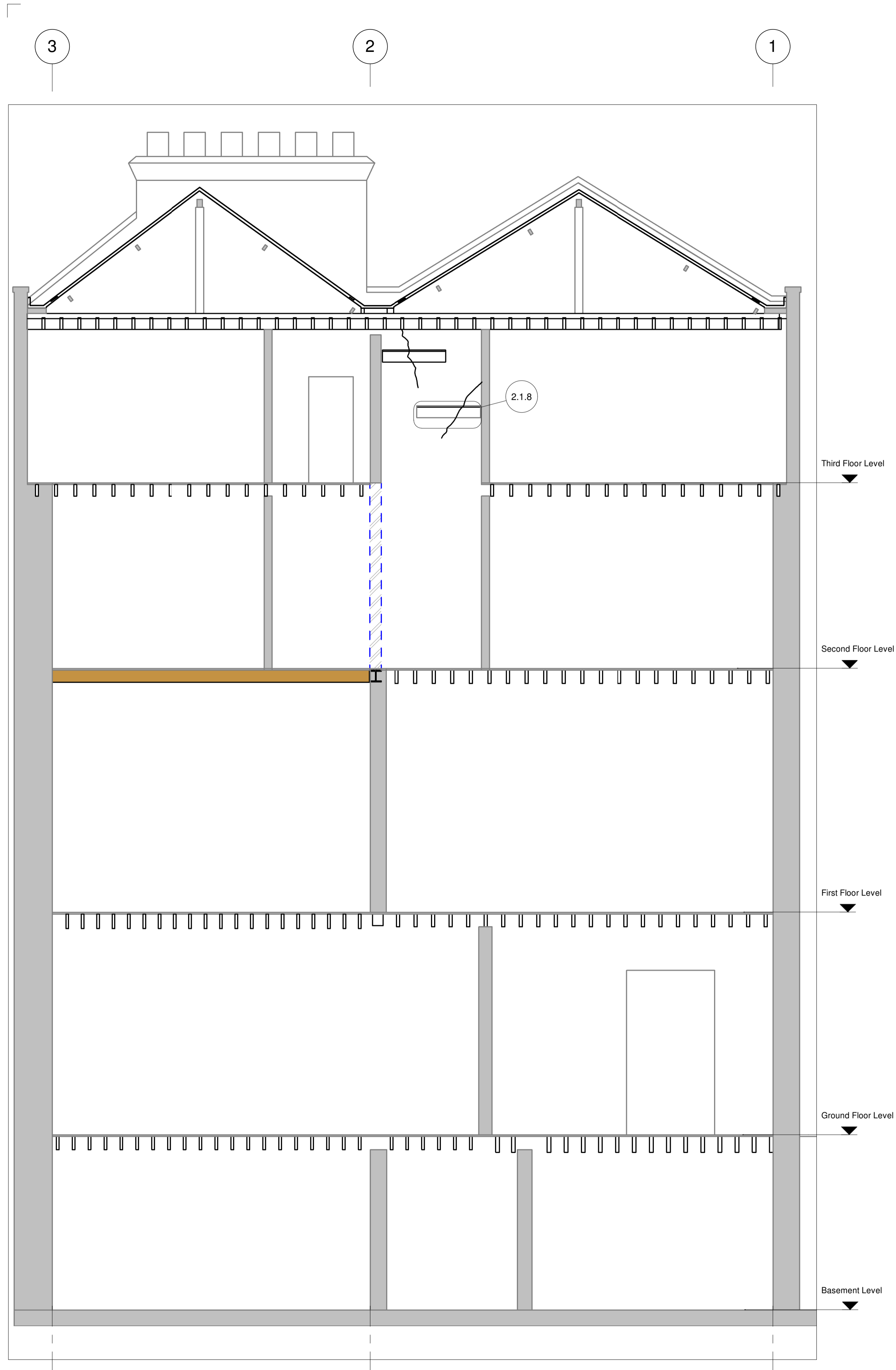
1 South Party Wall 1 : 50
