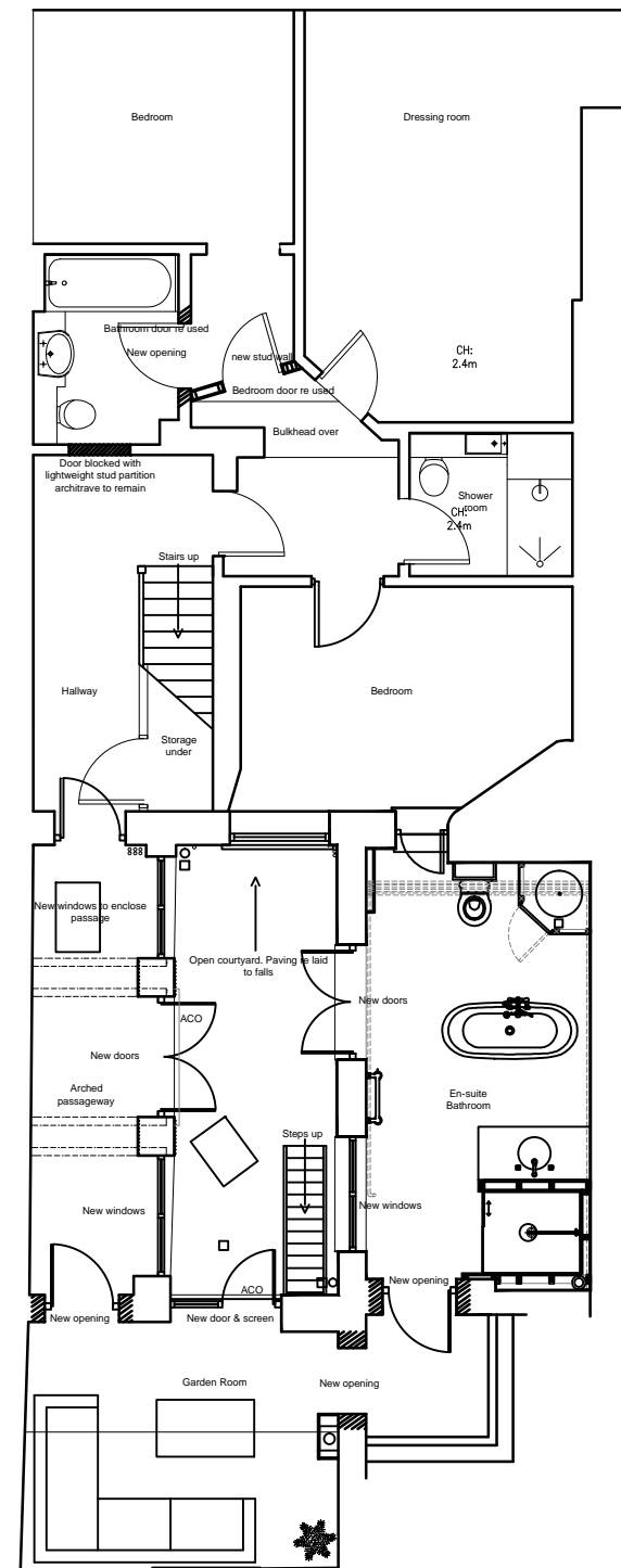
Proposed basement plan
