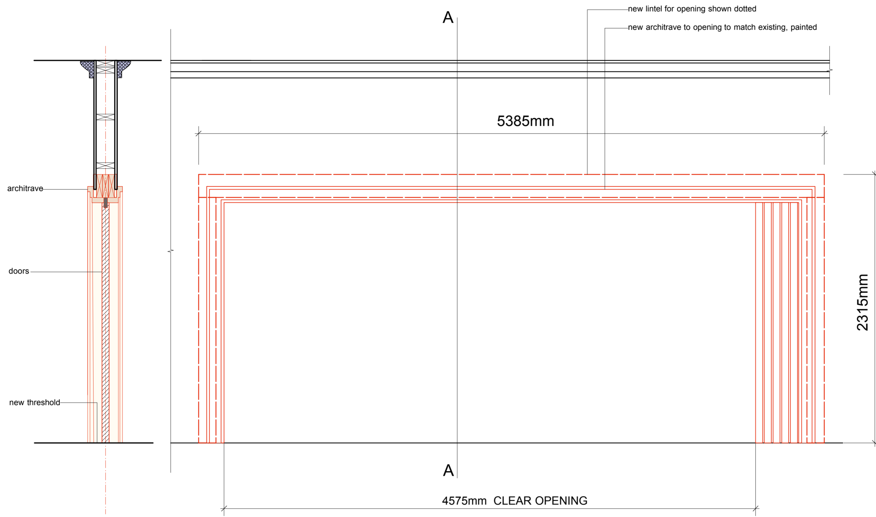
SECTION AA
