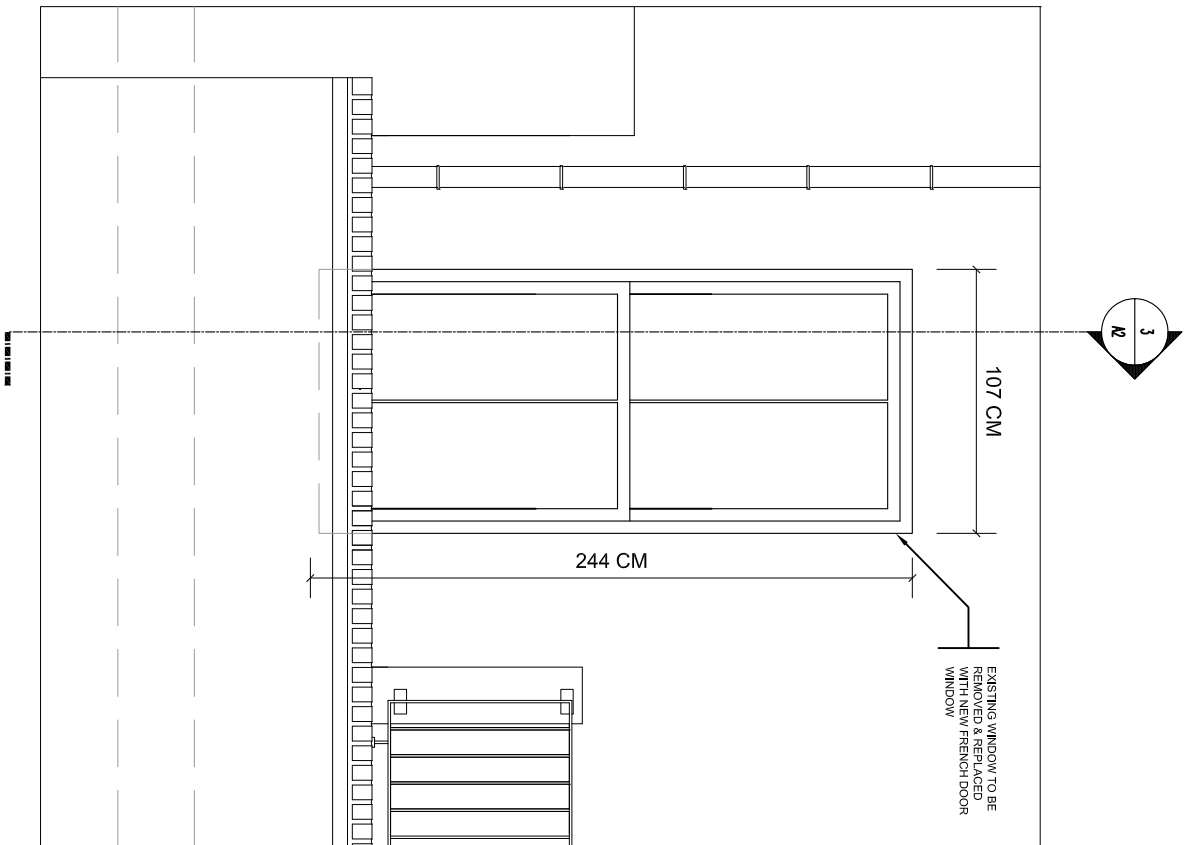
2 1:20 EXISTING TERRACE SOUTH ELEVATION
