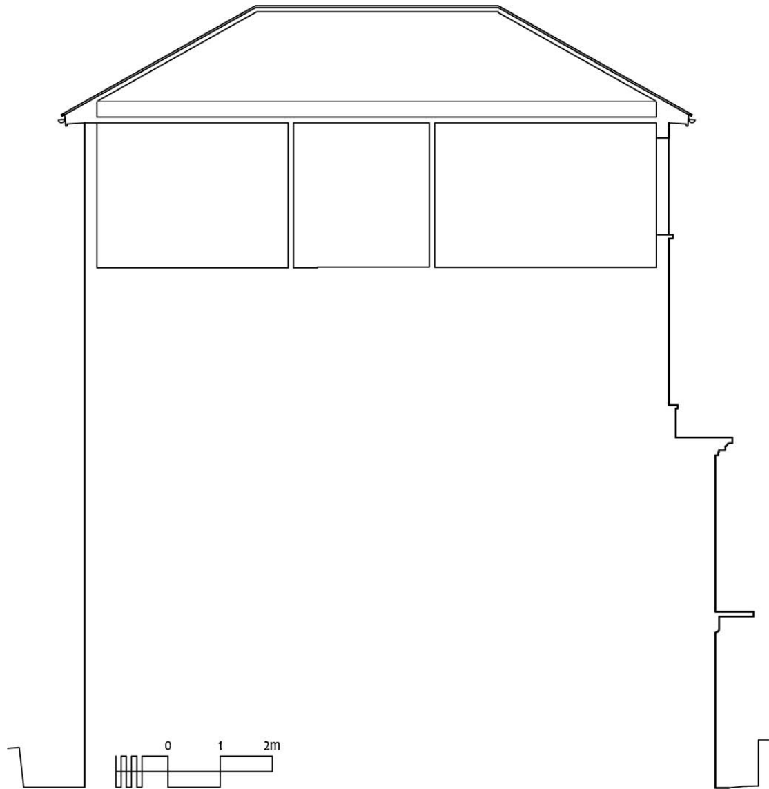
Section 1 – existing
