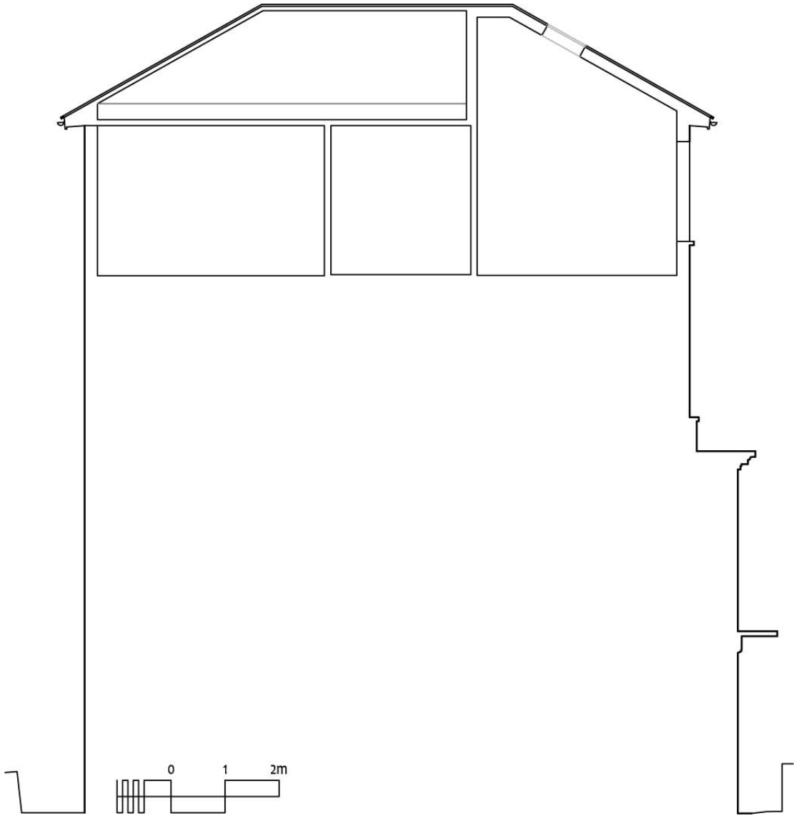
Section 1 – proposed
