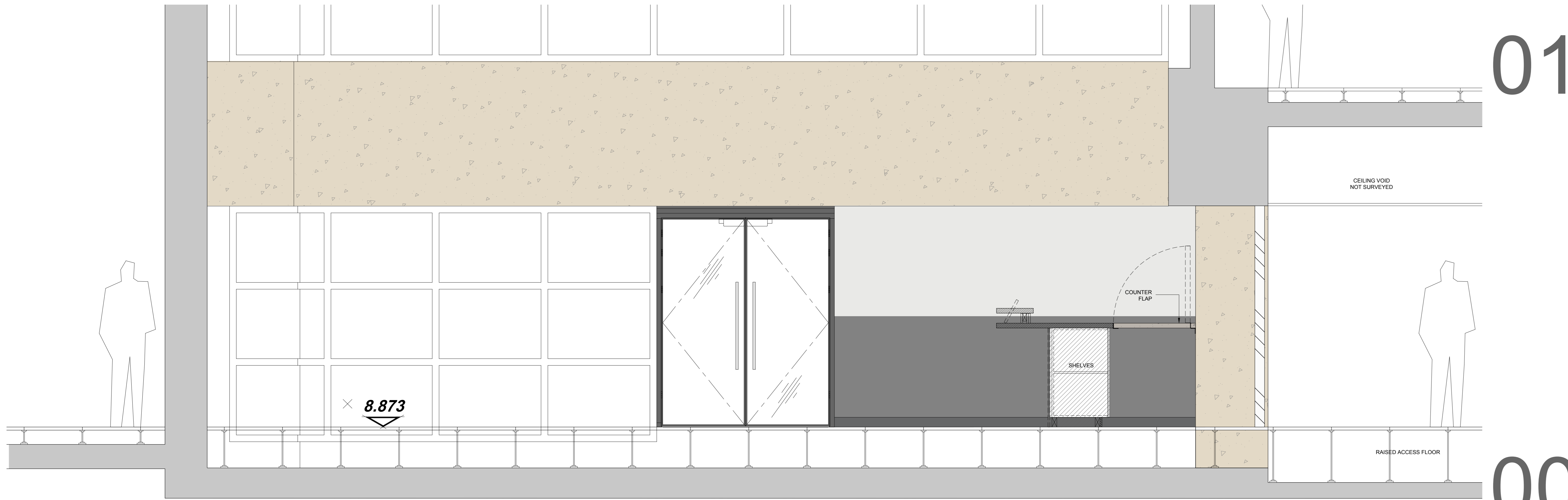
ATRIUM SECTION A SCALE 1:50
