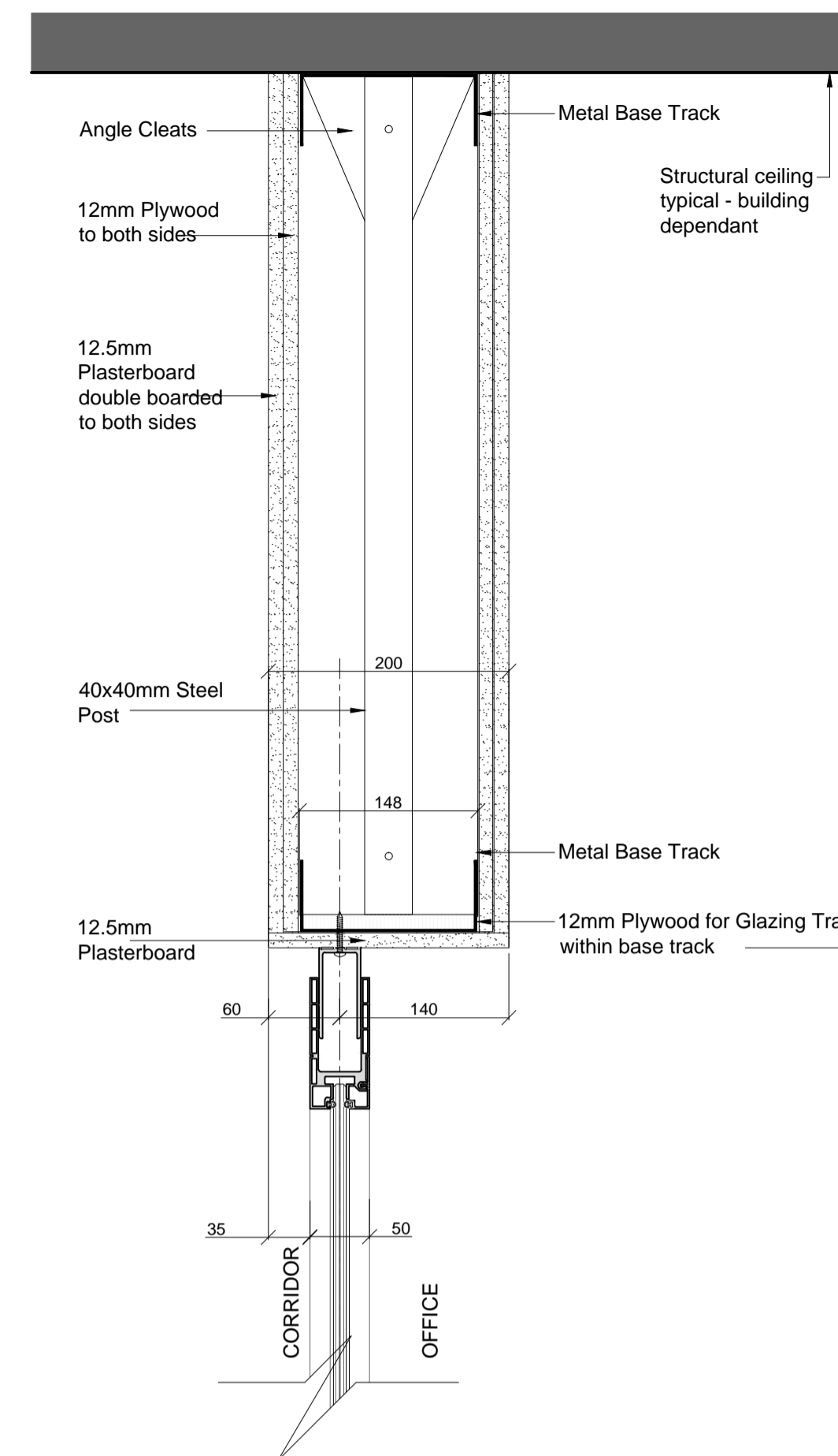
DETAIL P3 *showing partition corridor partitions (35mm offset with NO sliding door on corridor side)
