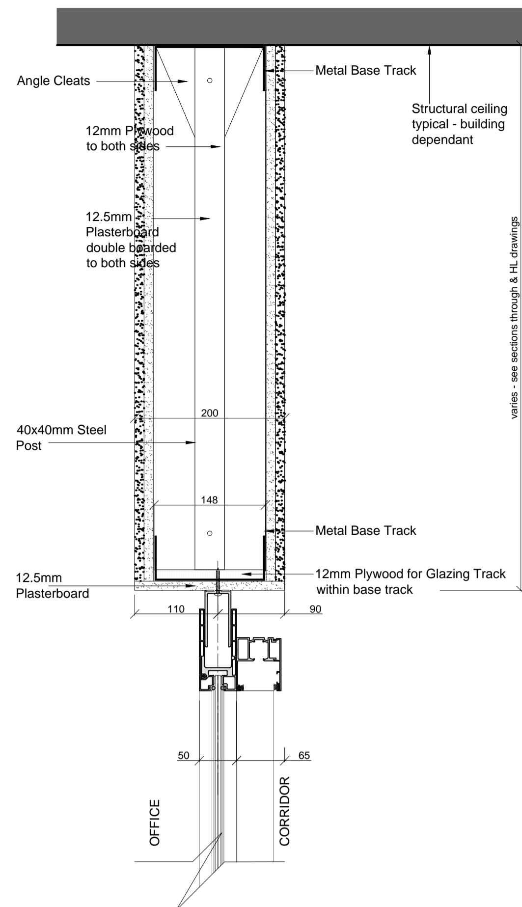
DETAIL P2 *showing partition corridor partitions (65mm offset with sliding doors on corridor side)
