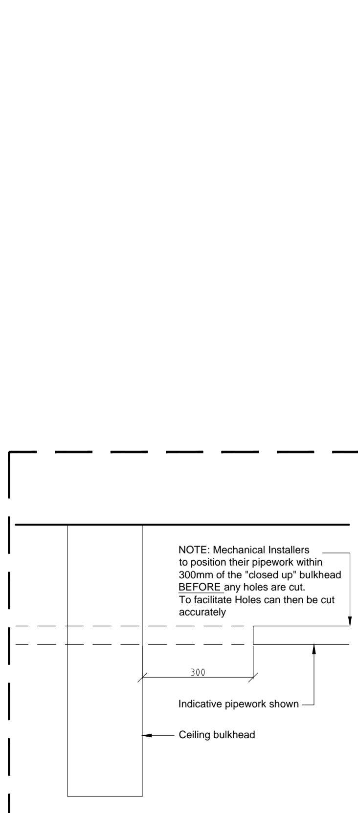
TYPICAL PIPEWORK PENETRATIONS SCALE 1:10
