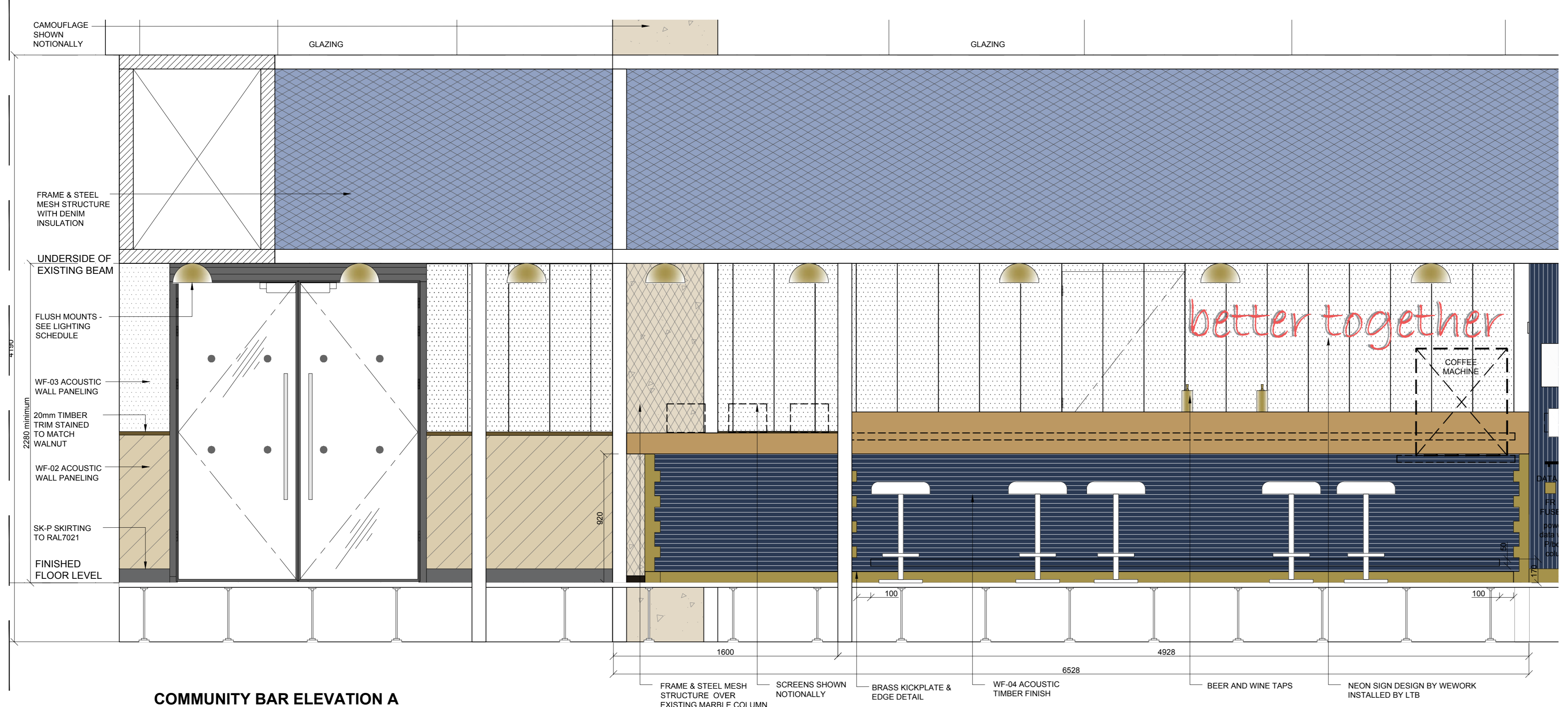
COMMUNITY BAR ELEVATION A SCALE 1:20
