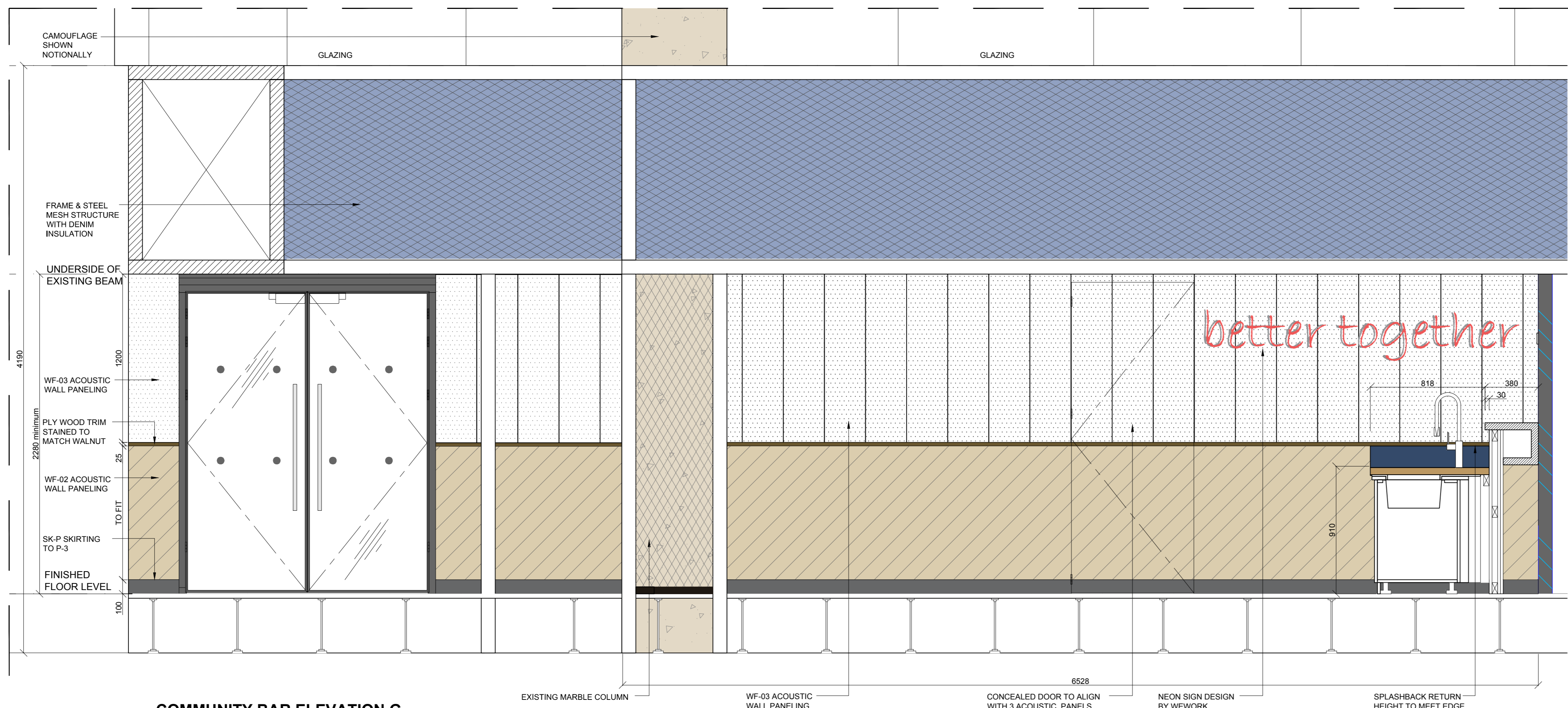
COMMUNITY BAR ELEVATION G SCALE 1:20
