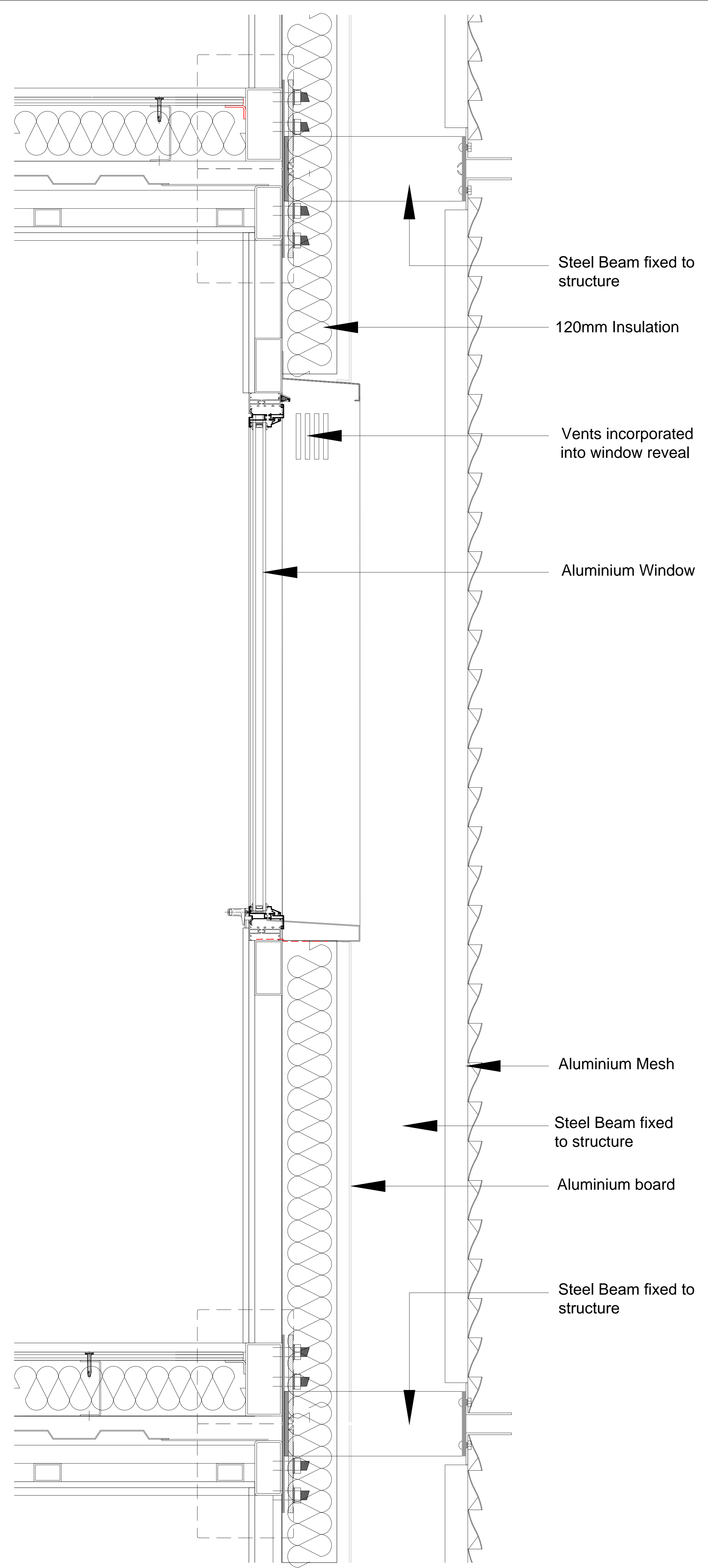
ALUMINIUM MESH FACADE SECTION DETAIL S. 1:5
