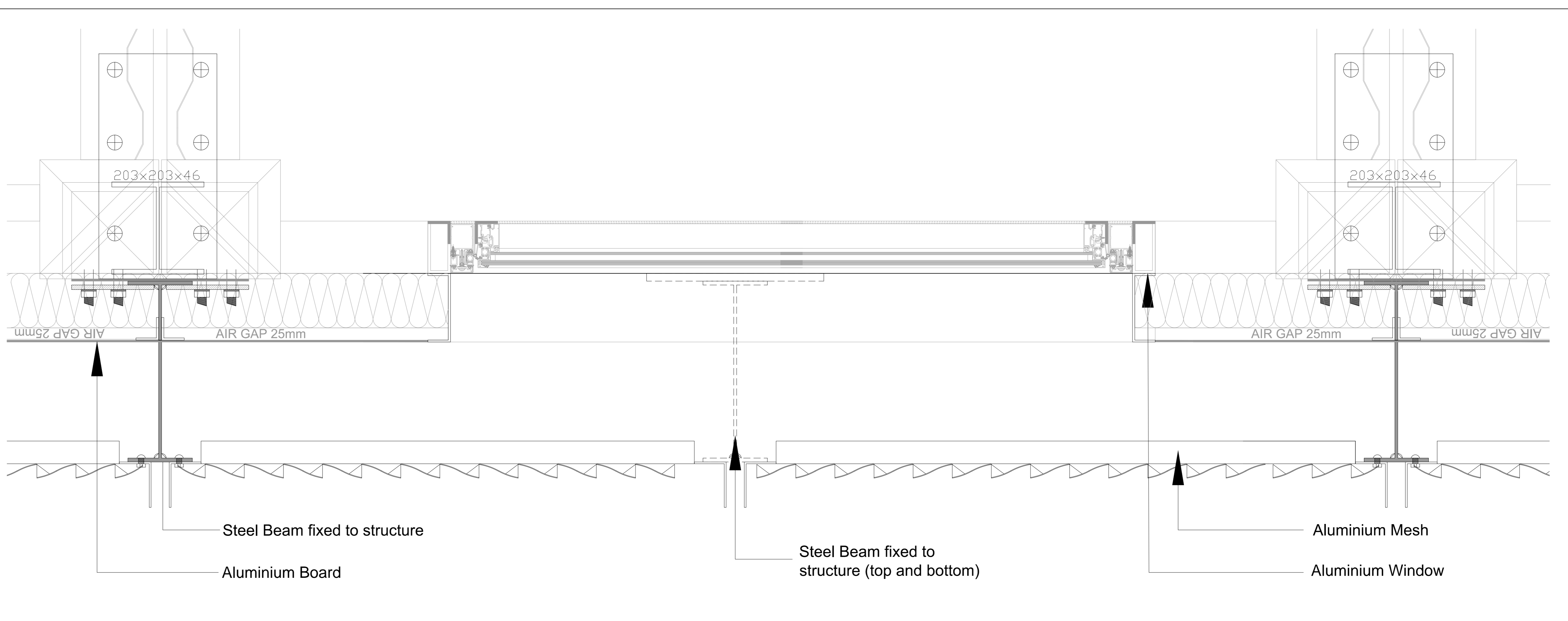
ALUMINIUM MESH FACADE PLAN DETAIL S. 1:5
