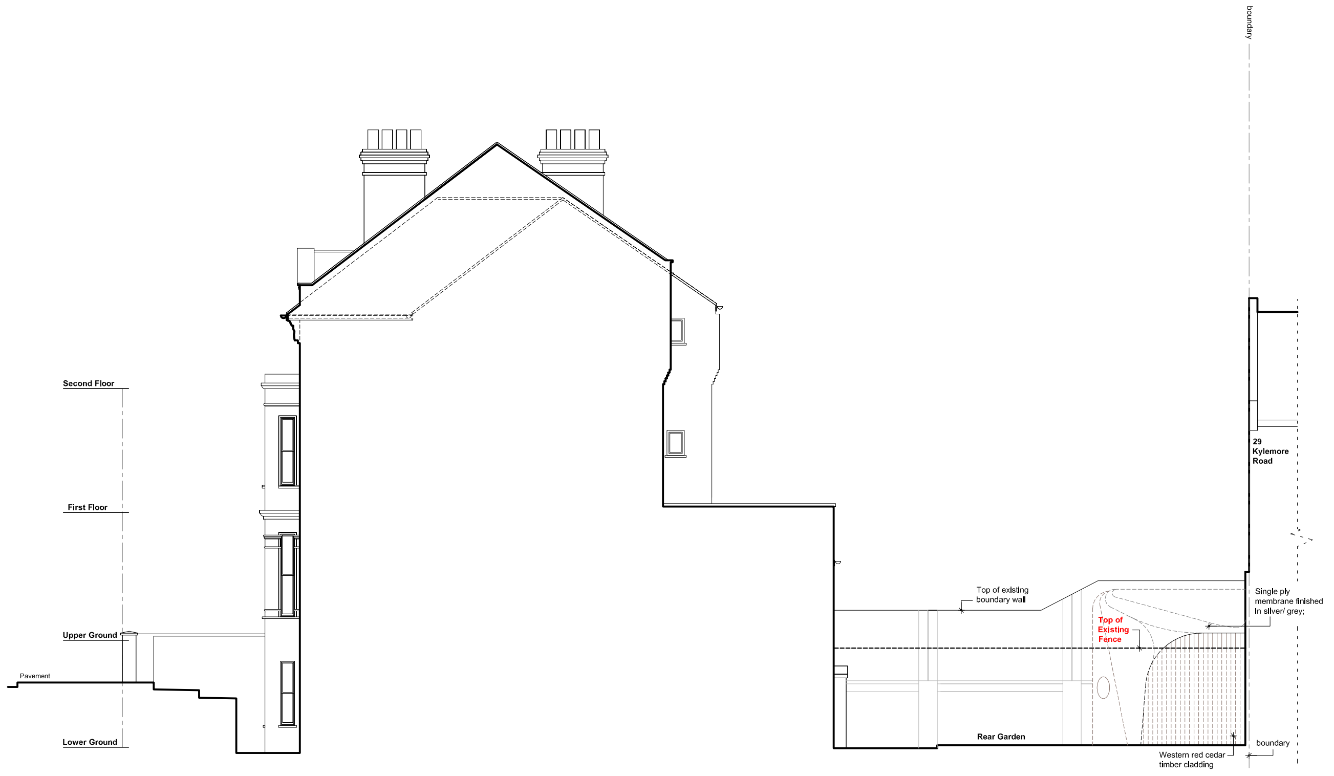
Proposed Side Elevation/ Section - East
