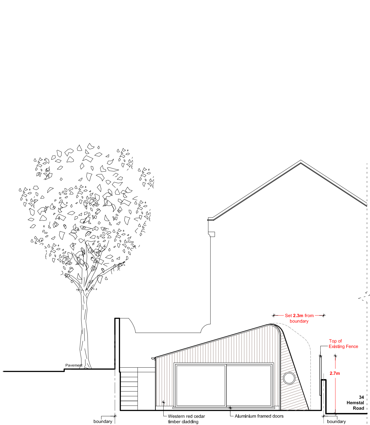
Proposed Elevation towards Garden Outbuilding - South
