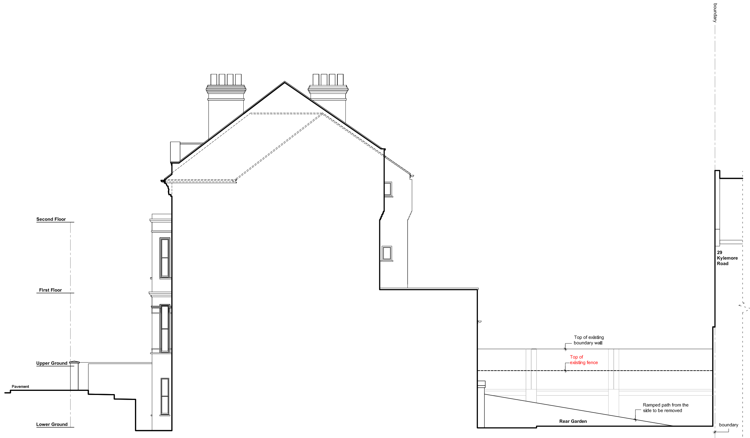
Existing Section Elevation - South/ North
