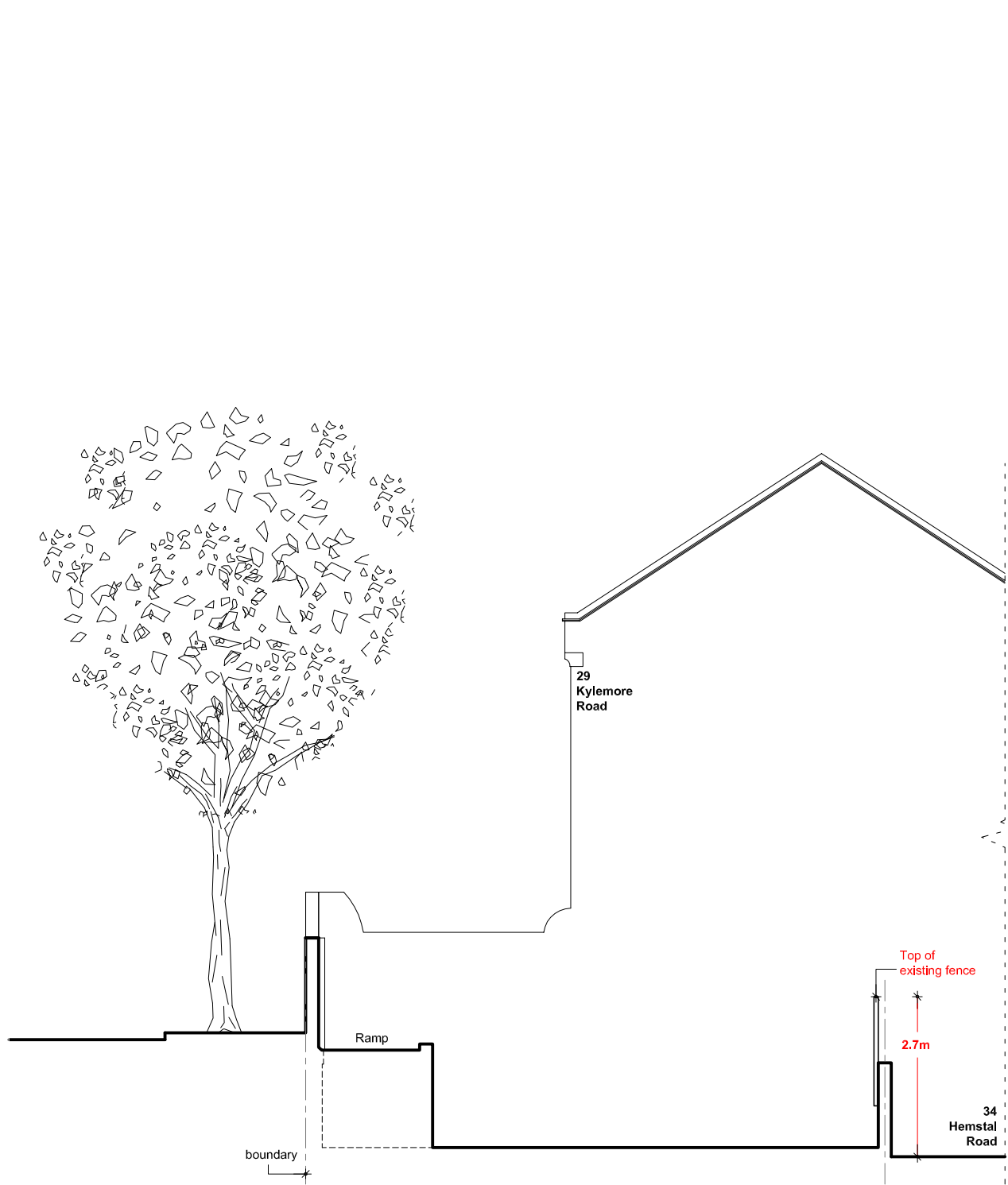
Existing Elevation towards Garden Outbuilding - South
