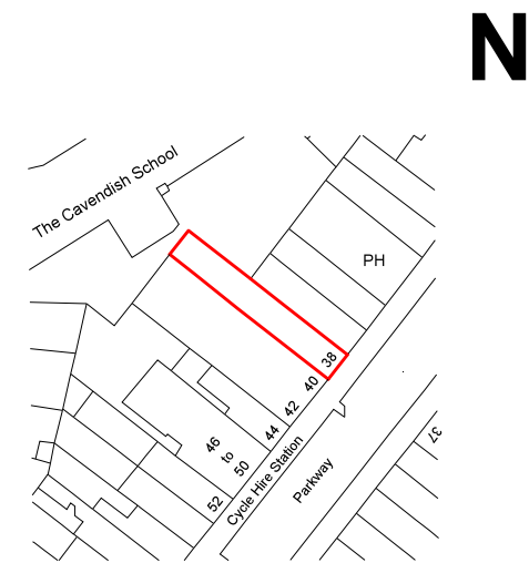
Site Location Plan Scale 1:1250
