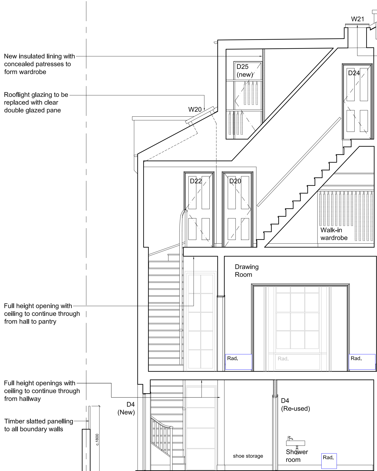
Section BB as Proposed Scale 1:50 @ A3
