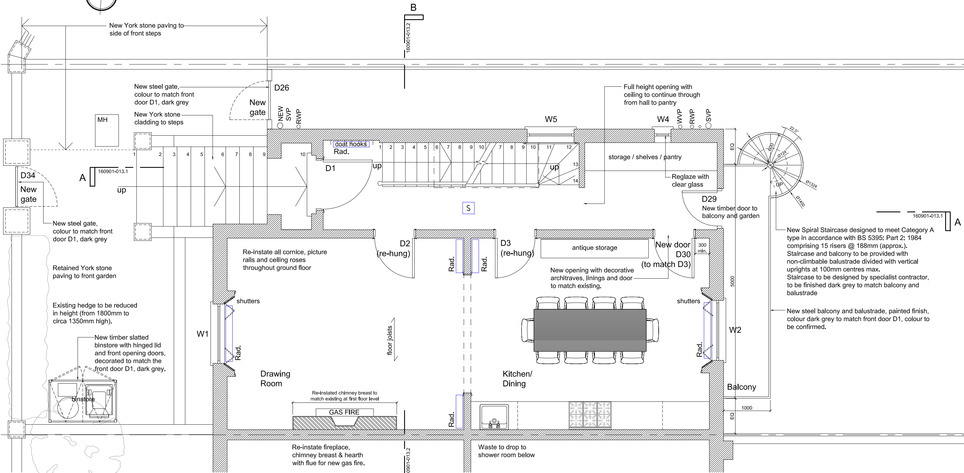
Ground Floor Plan as Proposed Scale 1:50 @ A3
