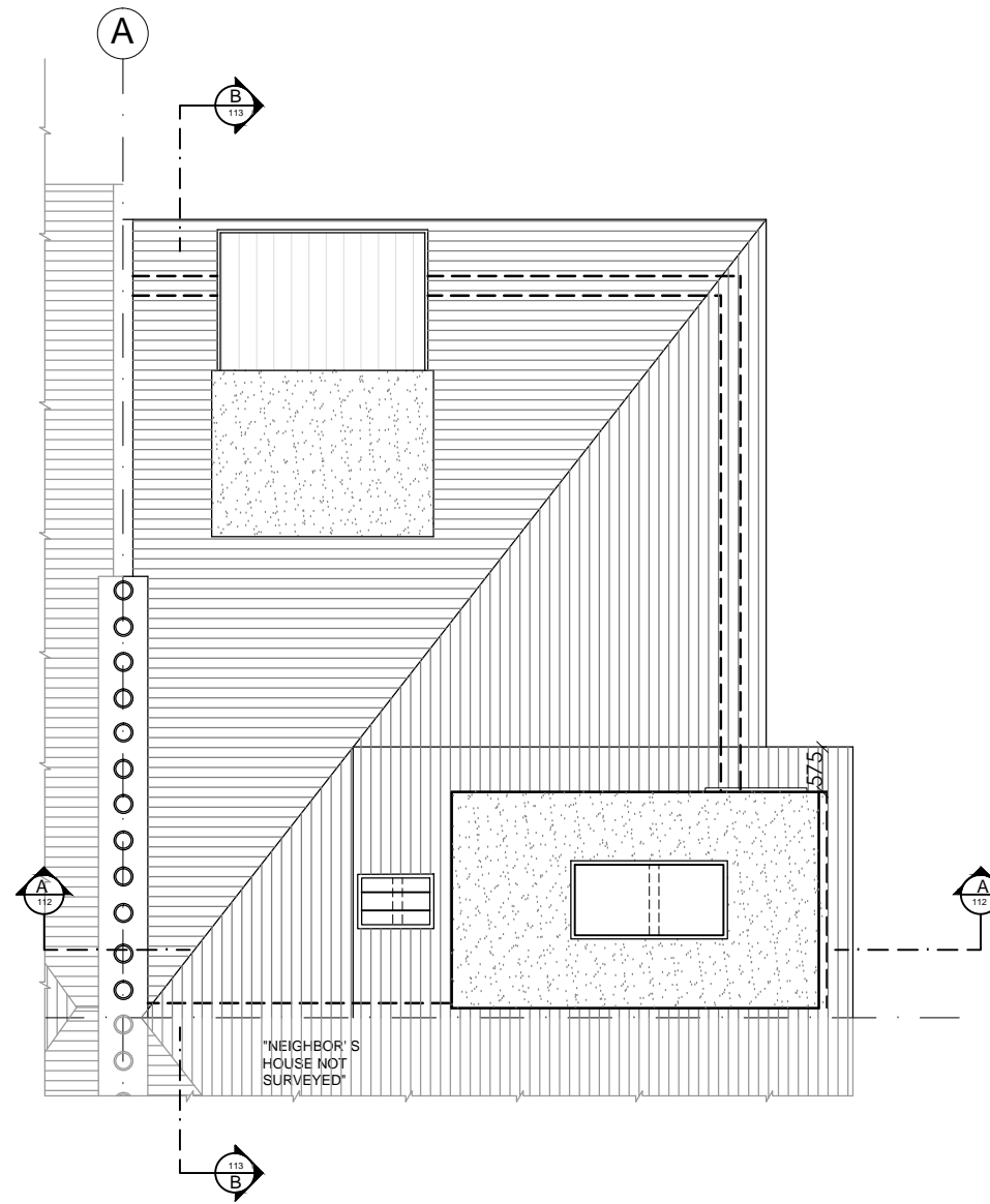
Roof Plan
