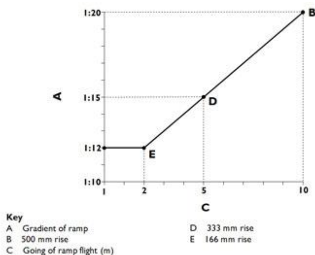
Figure 3.1 - Relationship between the gradient and going of a slope.
