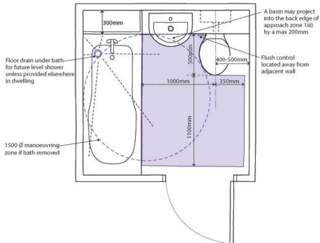
Figure 14b - Example bathroom layout
