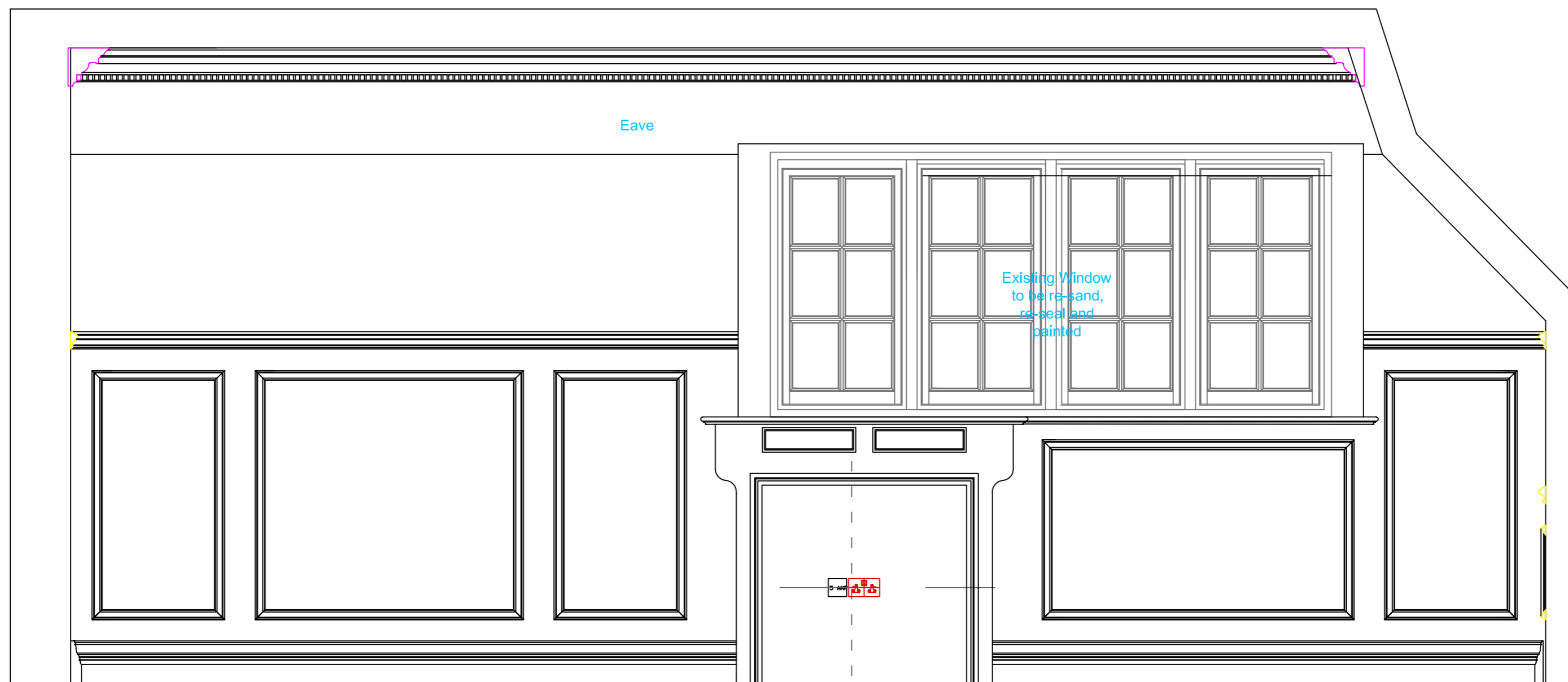
Elevation D - Existing
