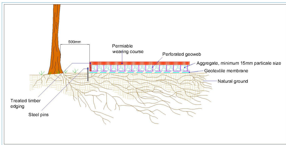
Typical cross section for multi-dimensional confinement system using timber edging
