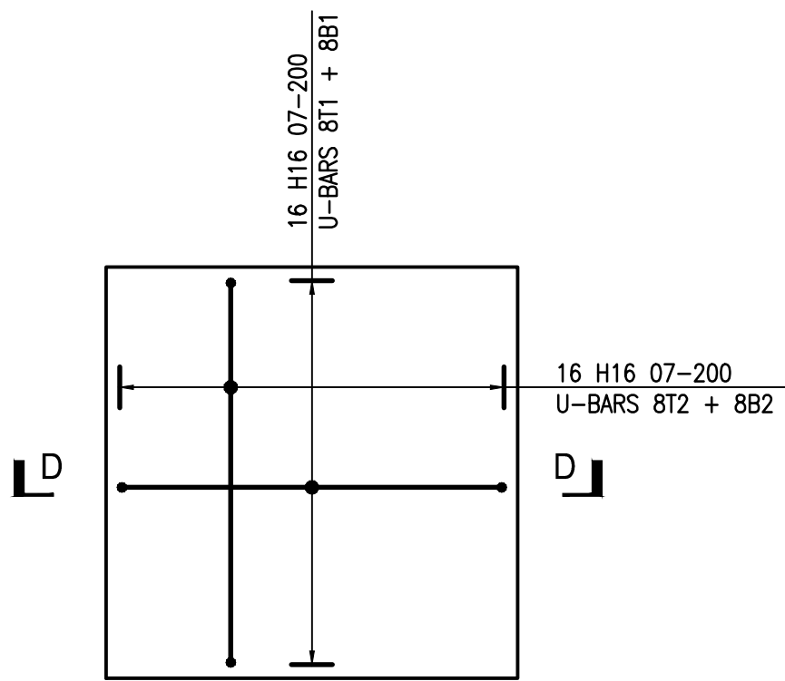
PAD FOOTING "P1" PLAN SCALE 1:25
