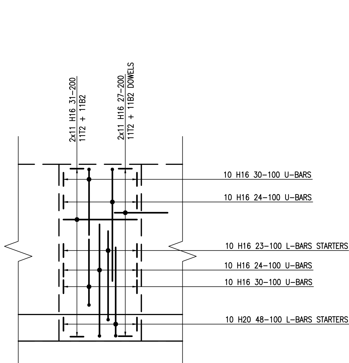
UNDERPINNING U.B PLAN 4 No. THUS SCALE 1:25
