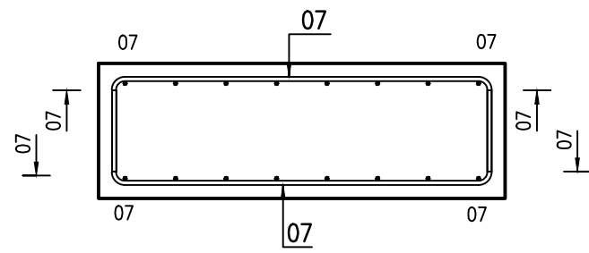
PAD FOOTING "P1" SECTION D-D SCALE 1:25
