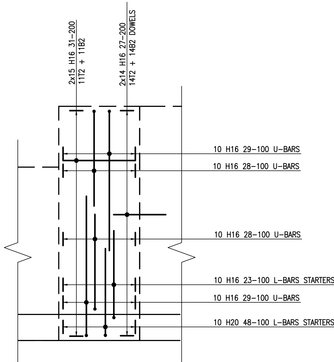
UNDERPINNING U.C PLAN 2 No. THUS SCALE 1:25
