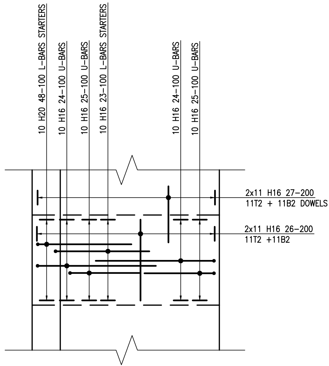
UNDERPINNING U.A PLAN 12 No. THUS SCALE 1:25
